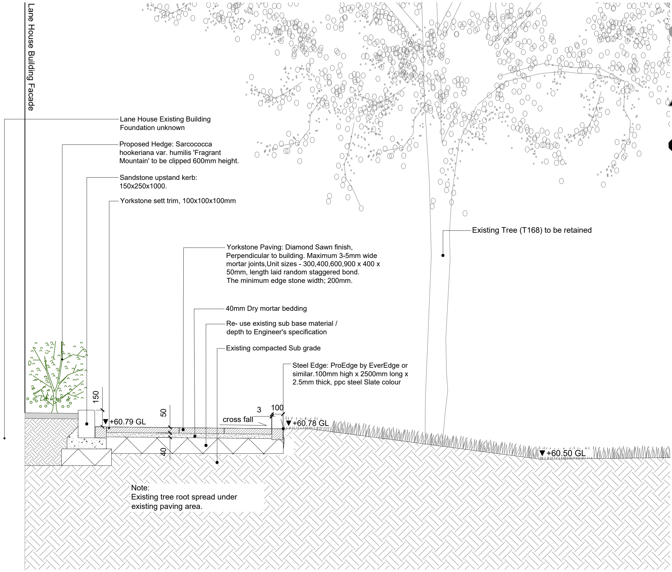
01 YORKSTONE PAVING WITH SETT TRIM 309 SECTION - NEAR EXISTING TREE SCALE 1:20
