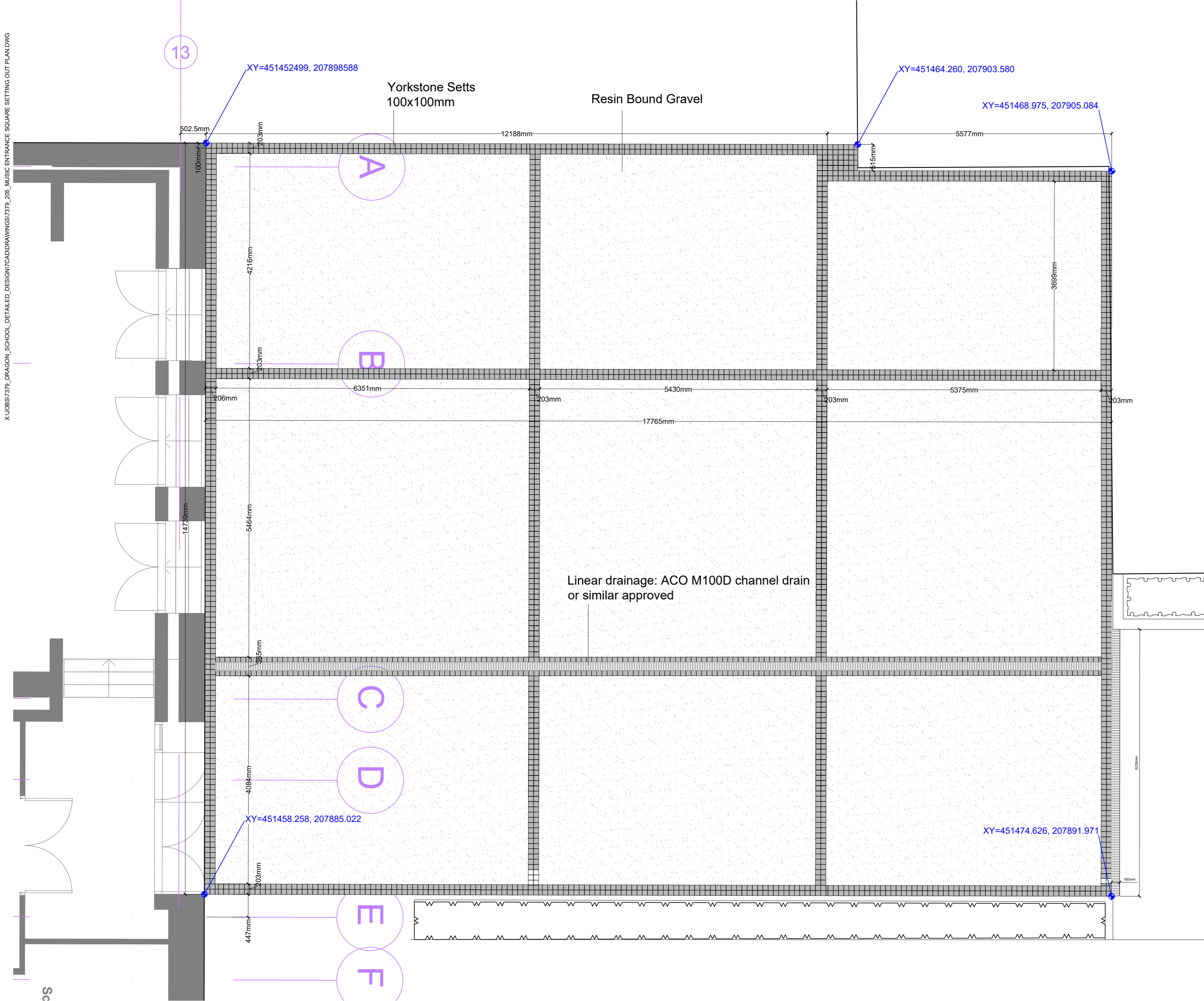
01 MUSIC ENTRANCE SQUARE PAVING PATTERN 205 PLAN SCALE 1:50
