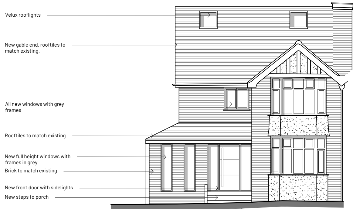
FRONT ELEVATION (WEST FACING)
