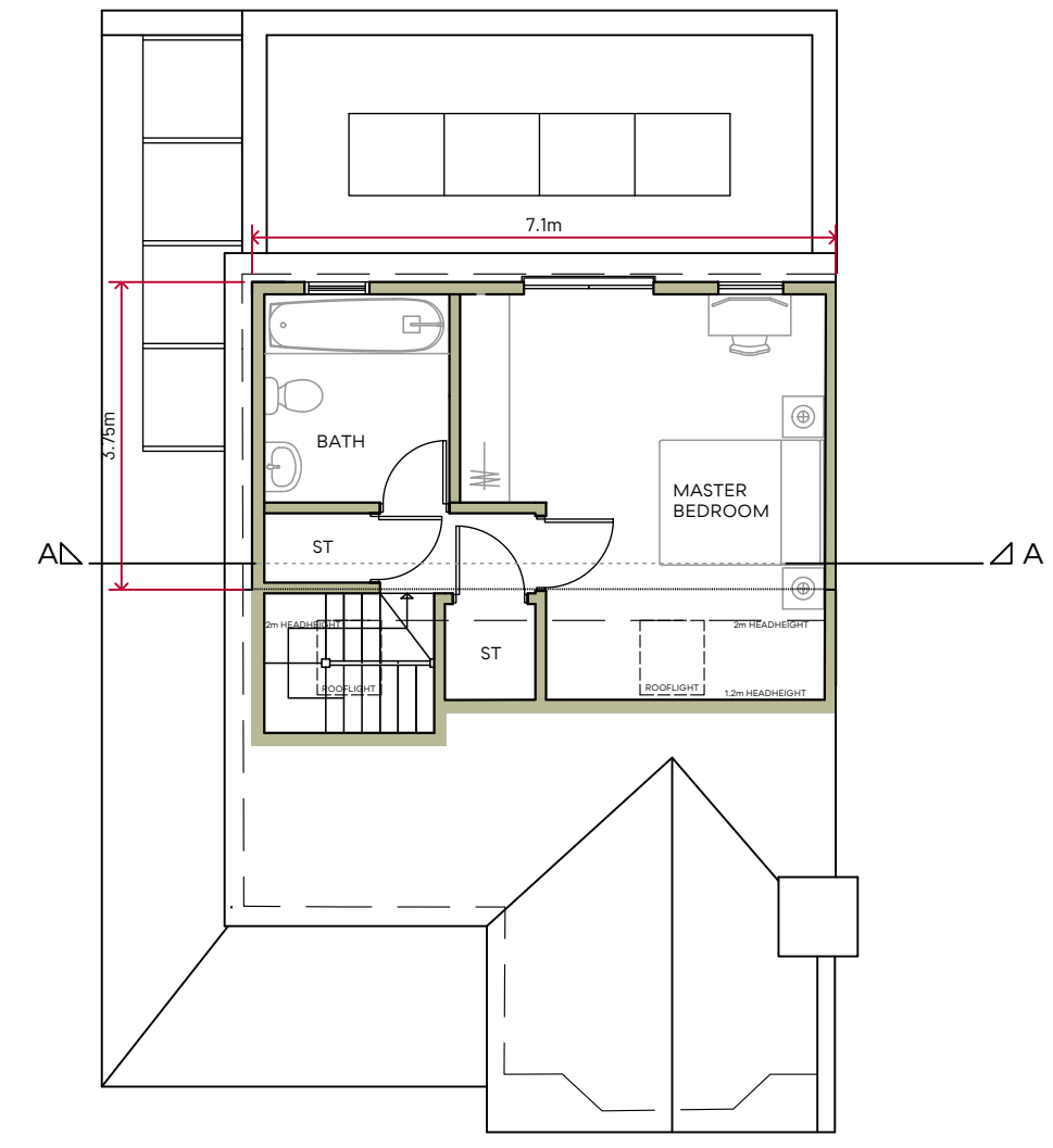
LOFT PLAN @ 1:100
