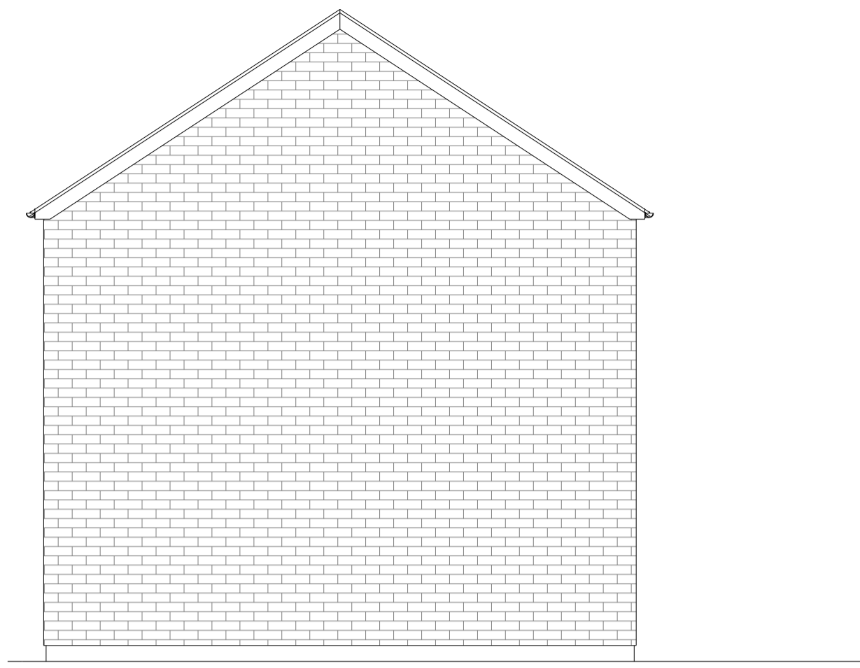
Existing South-east Elevation (Existing North-west Elevation is a Mirror Image)
