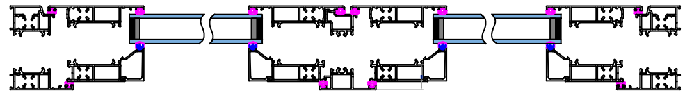
Horizontal section DD Scale 1/5 @ A3
