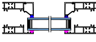
Horizontal section BB Scale 1/5 @ A3
