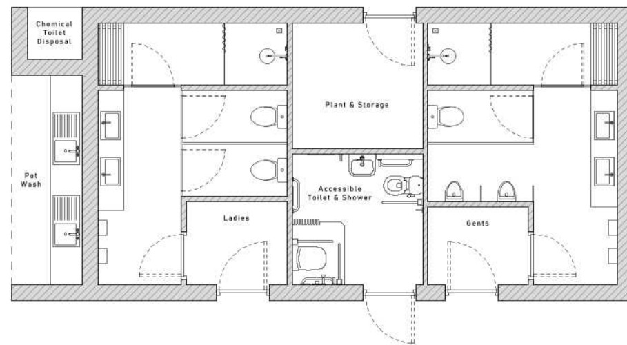
FLOOR PLAN
