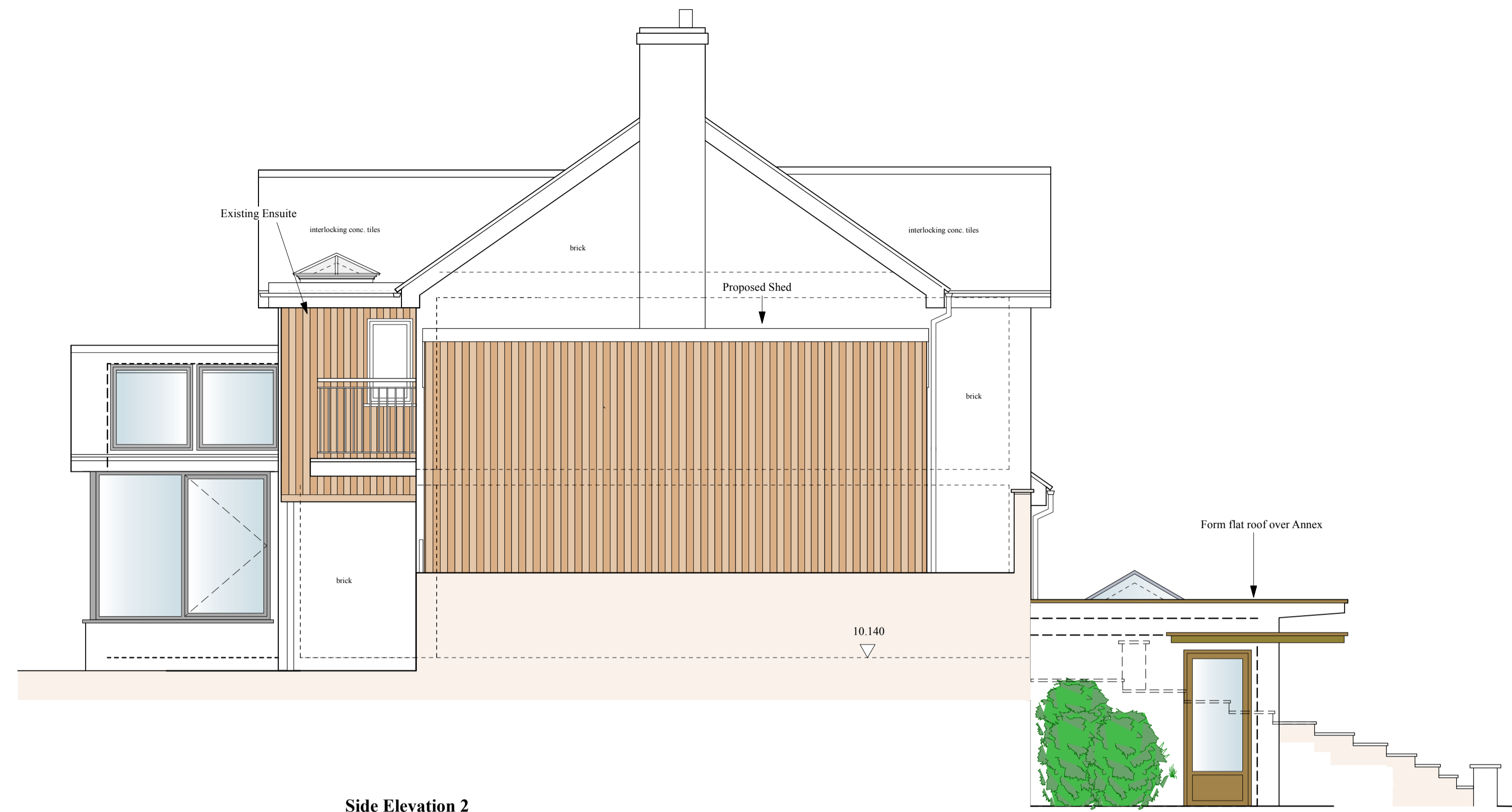
Side Elevation 2
