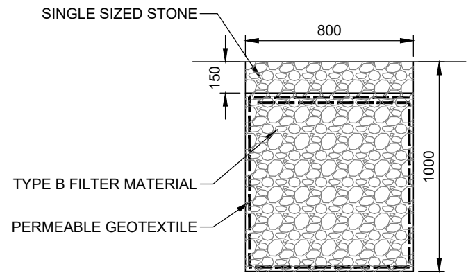
CUT OFF DRAIN SCALE 1:25
