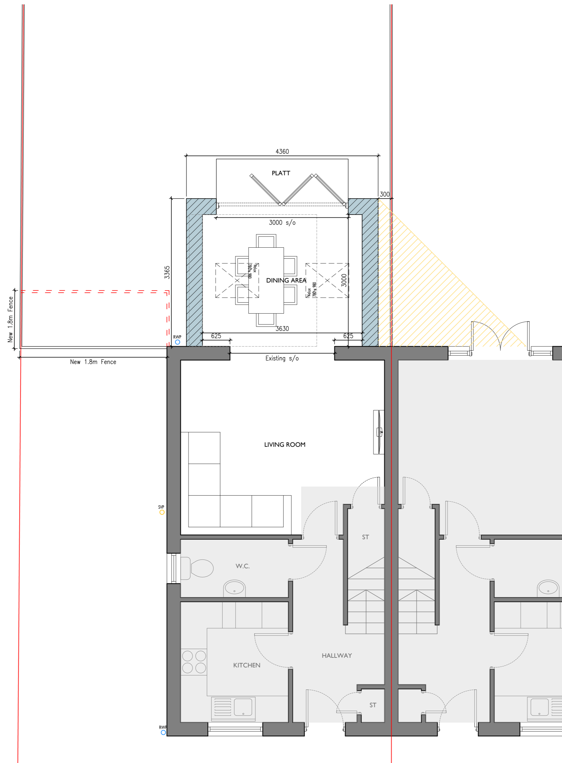
Proposed Ground Floor Plan (Option I) 1:50 Area: 14.6 m2 approx
