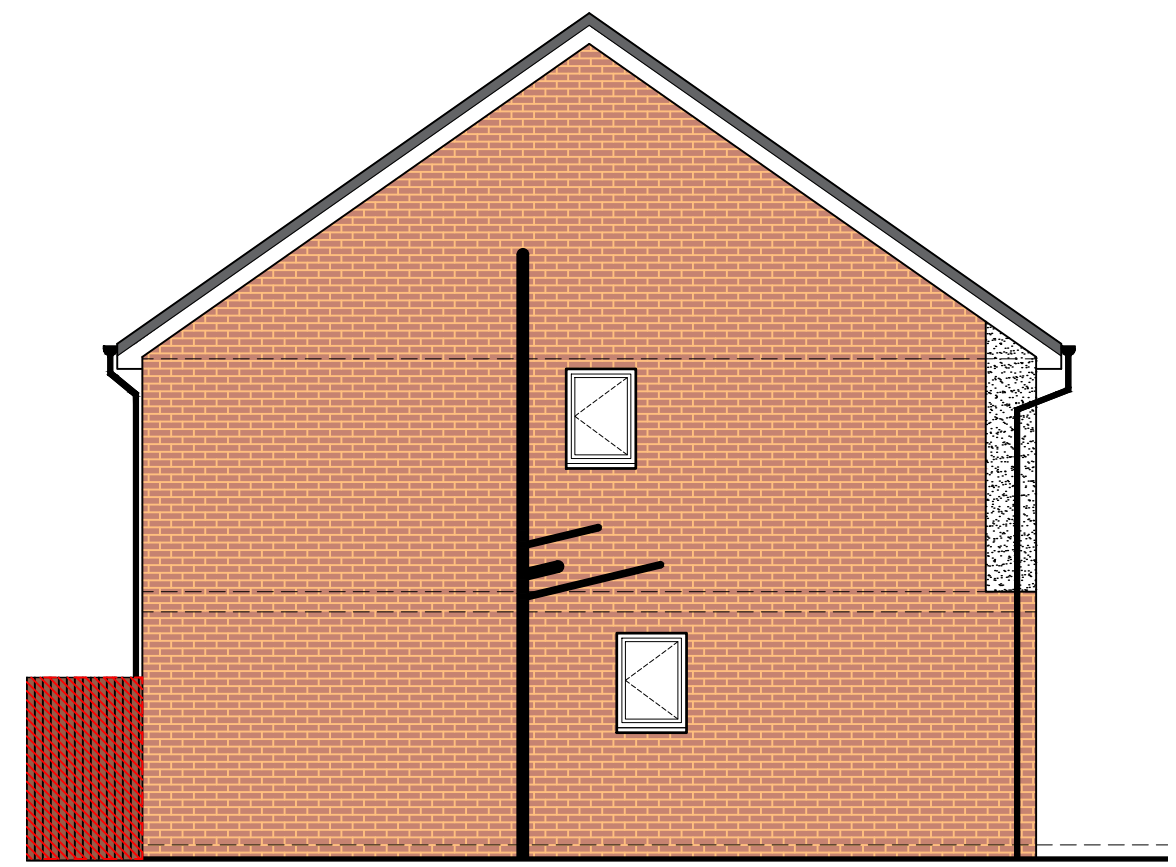
Existing Side Elevation 1:75
