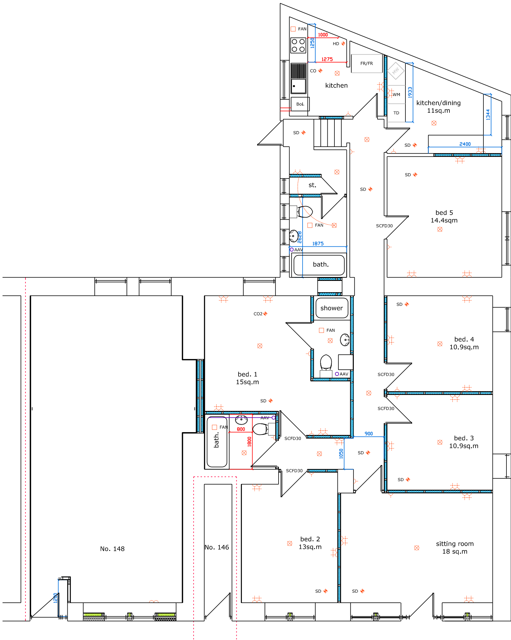
ground floor layout 1:75
