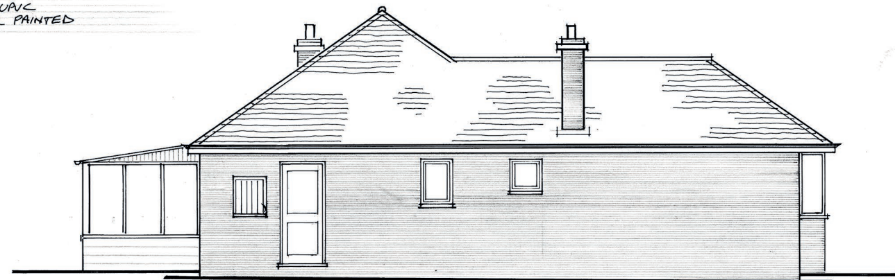
SIDE [NORTH] ELEVATION.
