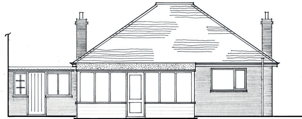
REAR [EAST] ELEVATION.
