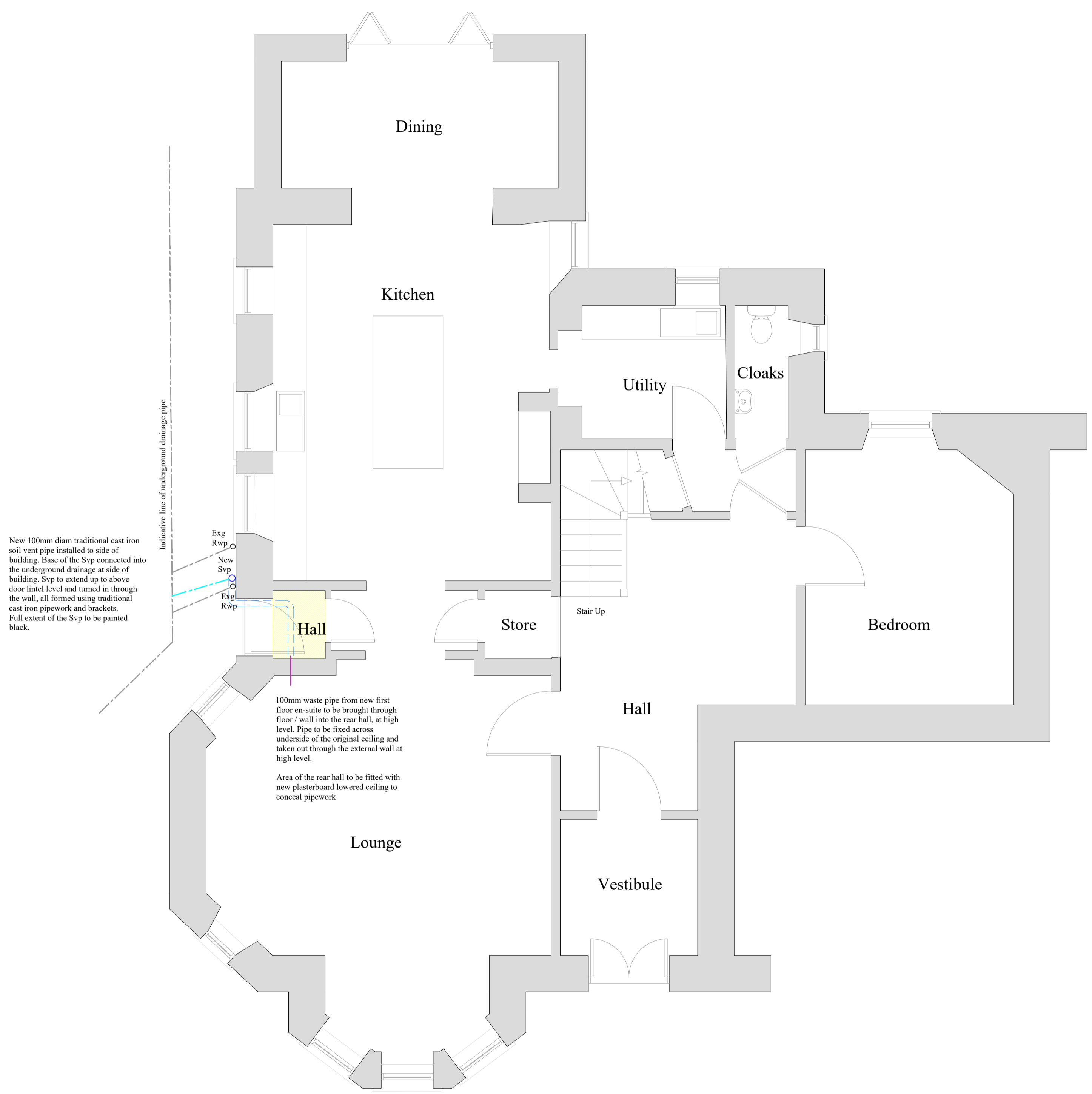
1:50 GROUND FLOOR PLAN AS PROPOSED
