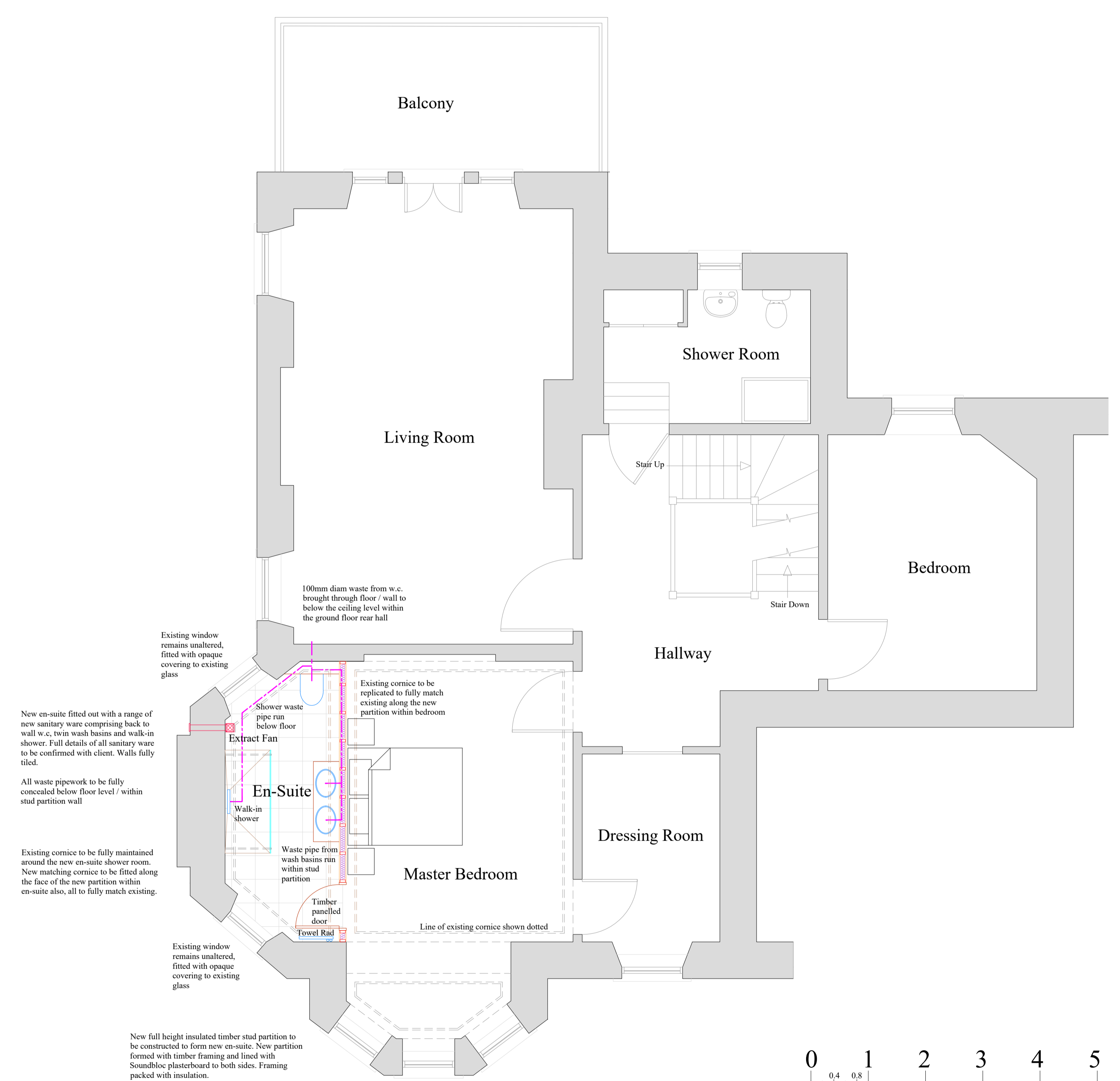
1:50 FIRST FLOOR PLAN AS PROPOSED
