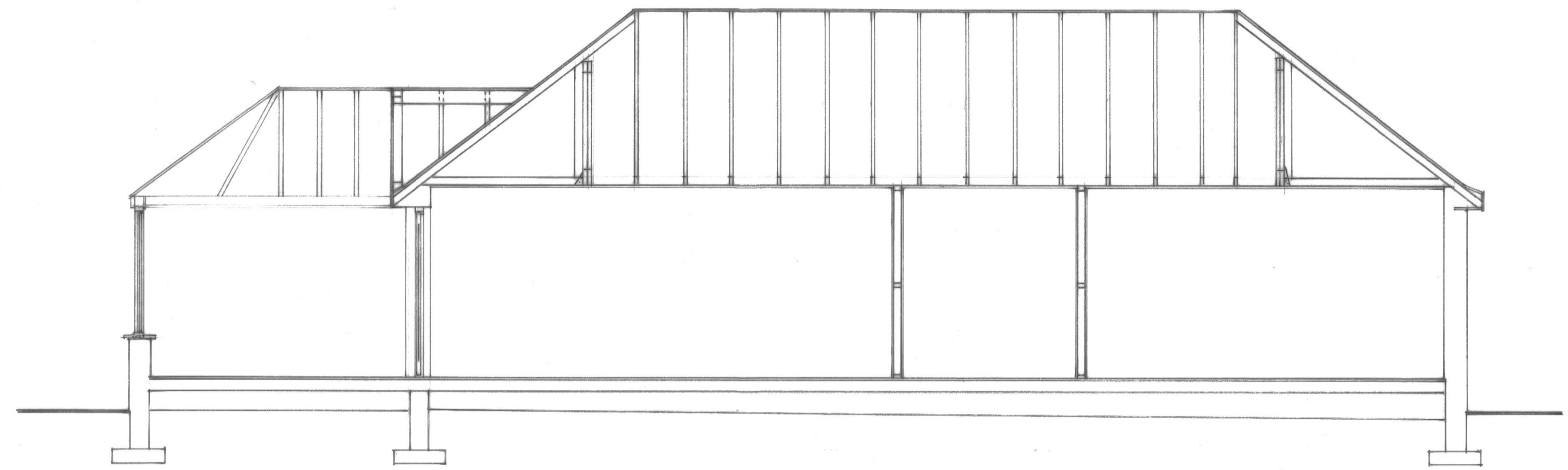
EXISTING SECTION
