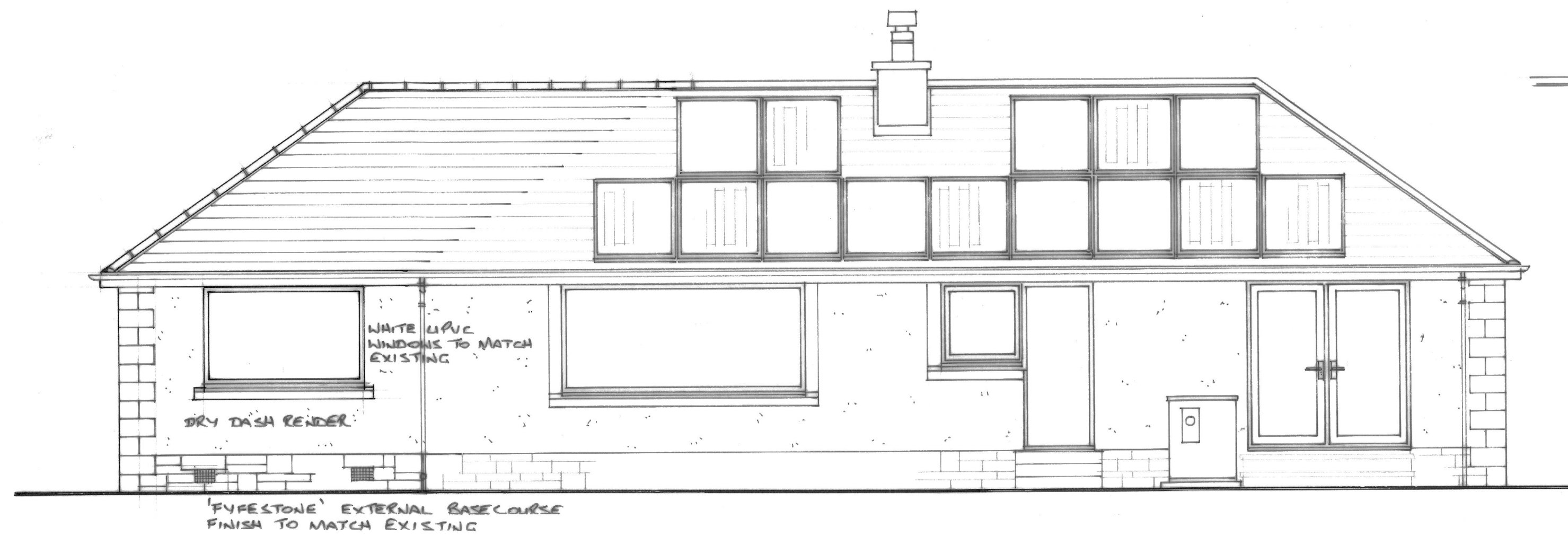
PROPOSED SIDE ELEVATION (west)
