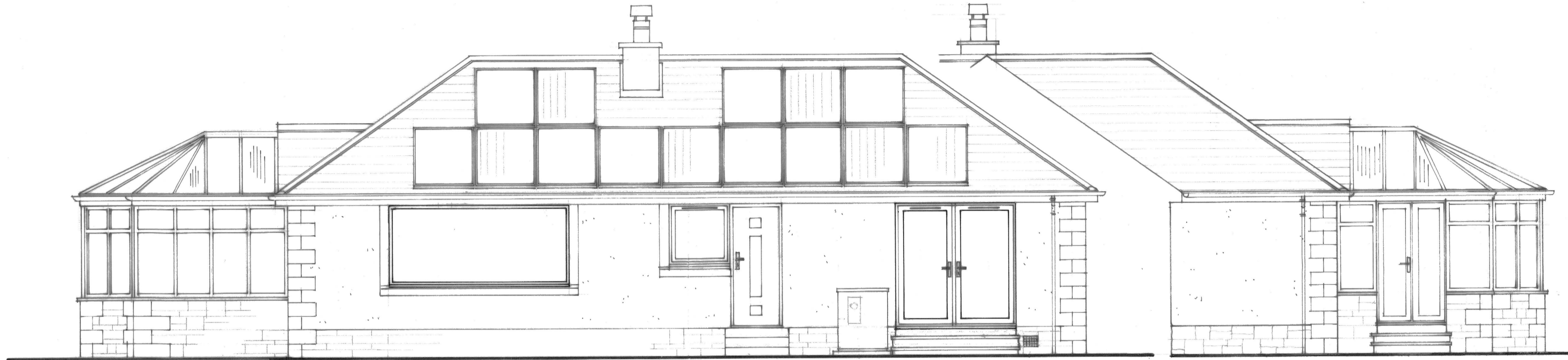
EXISTING SIDE ELEVATION (as viewed from courtyard)
