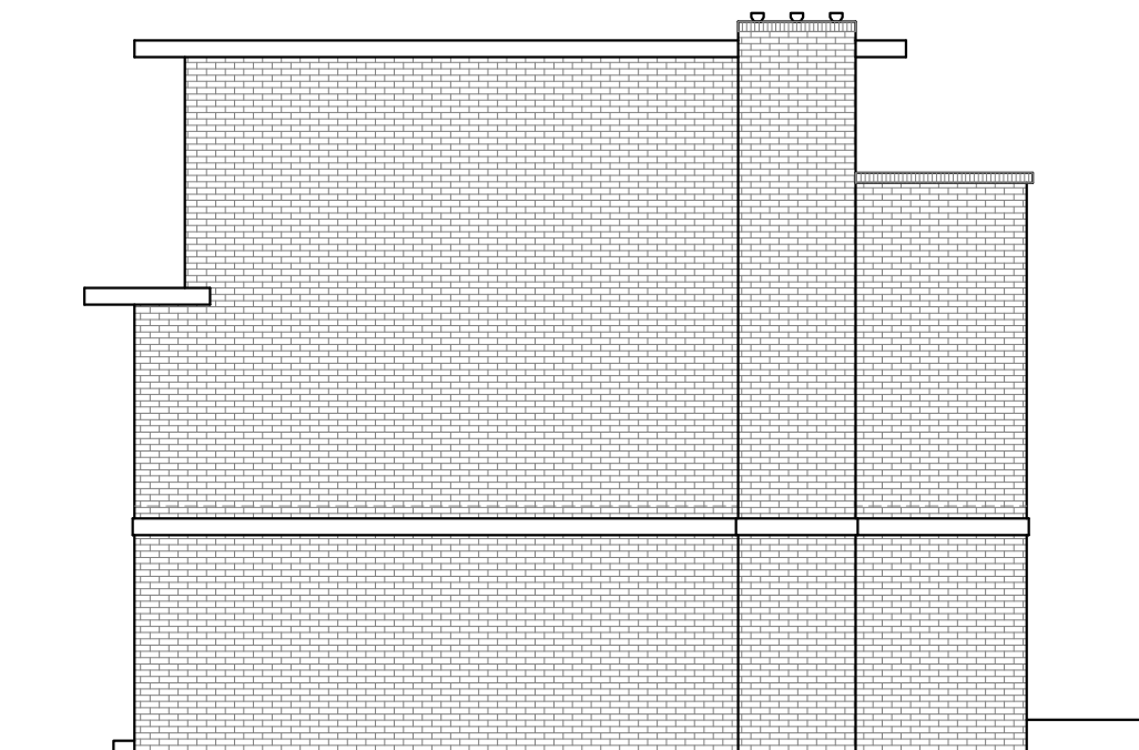
PROPOSED NORTH SIDE ELEVATION SCALE= 1:100
