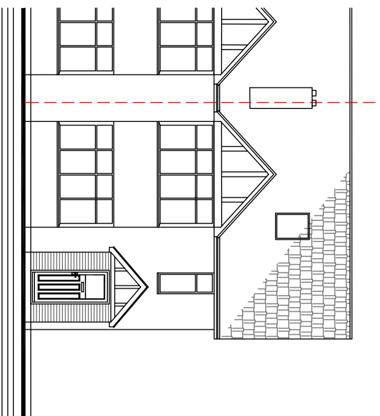
North Elevation
