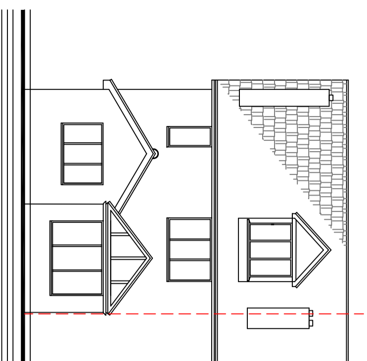
South Elevation
