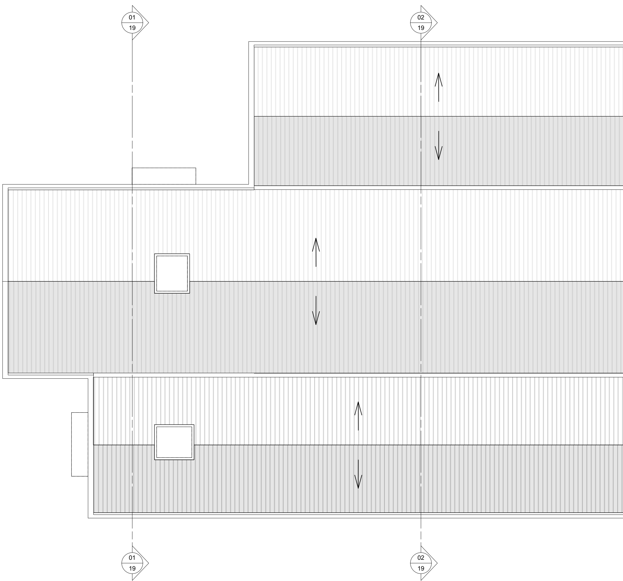
01 Proposed Roof Plan 15 1:200@A3; 1:100@A1
