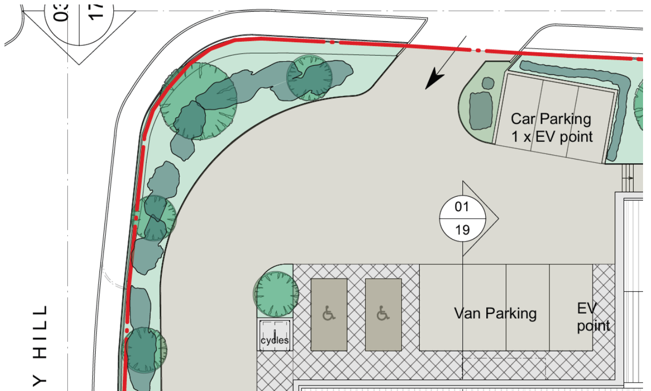
External Cycle Store – Sheffield stand for 2 cycles with proprietary cycle shelter with roof and sides clad in PETG-UV clear sheet over steel frame.
