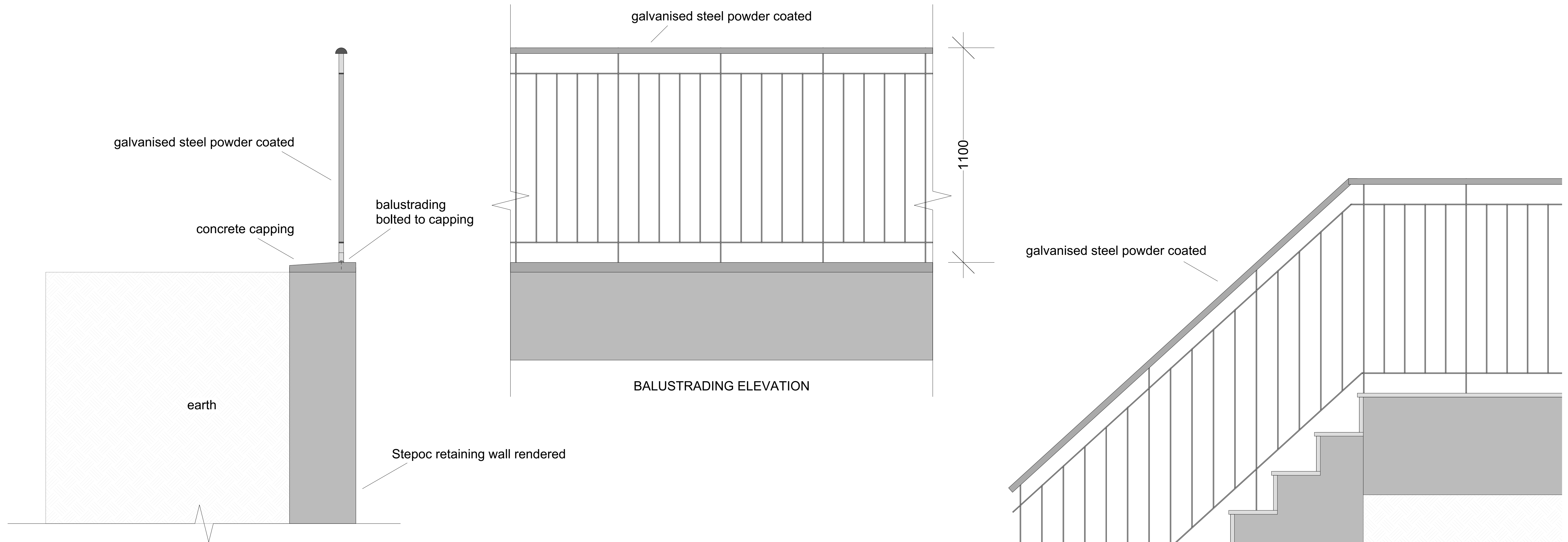
BALUSTRADING SECTION ON RETAINING WALLS
