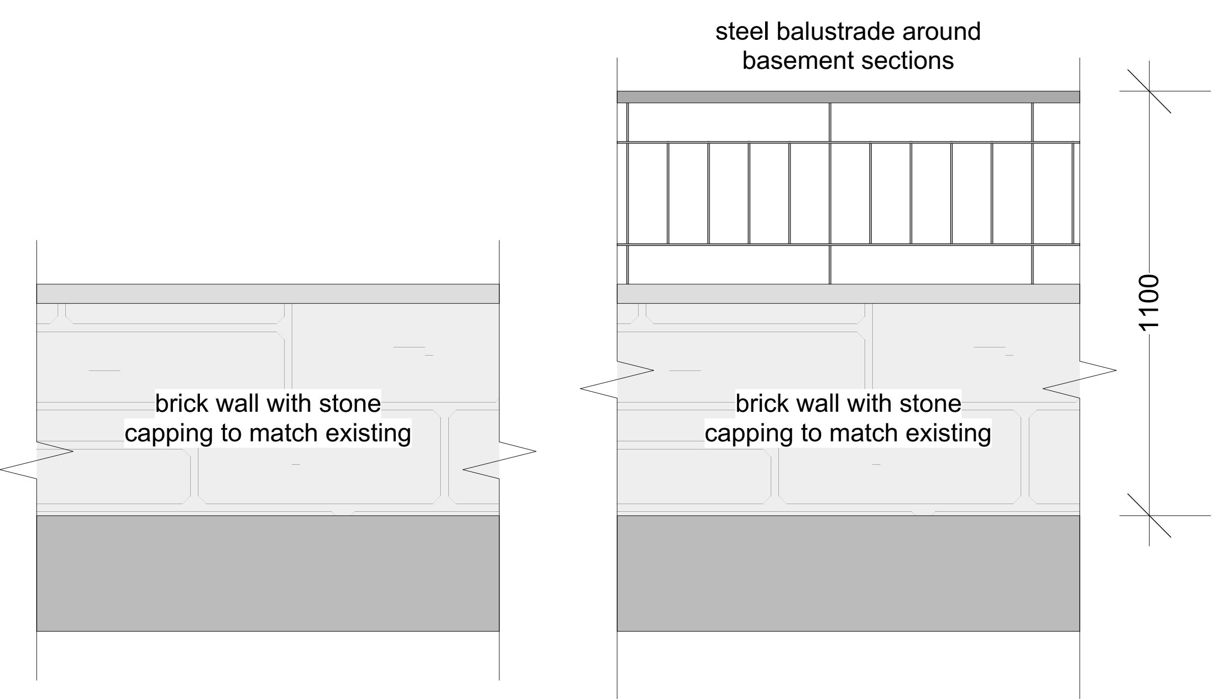
LOW LEVEL BOUNDARY WALL ALONG GLOUCESTER RD AND Highbury ROAD
