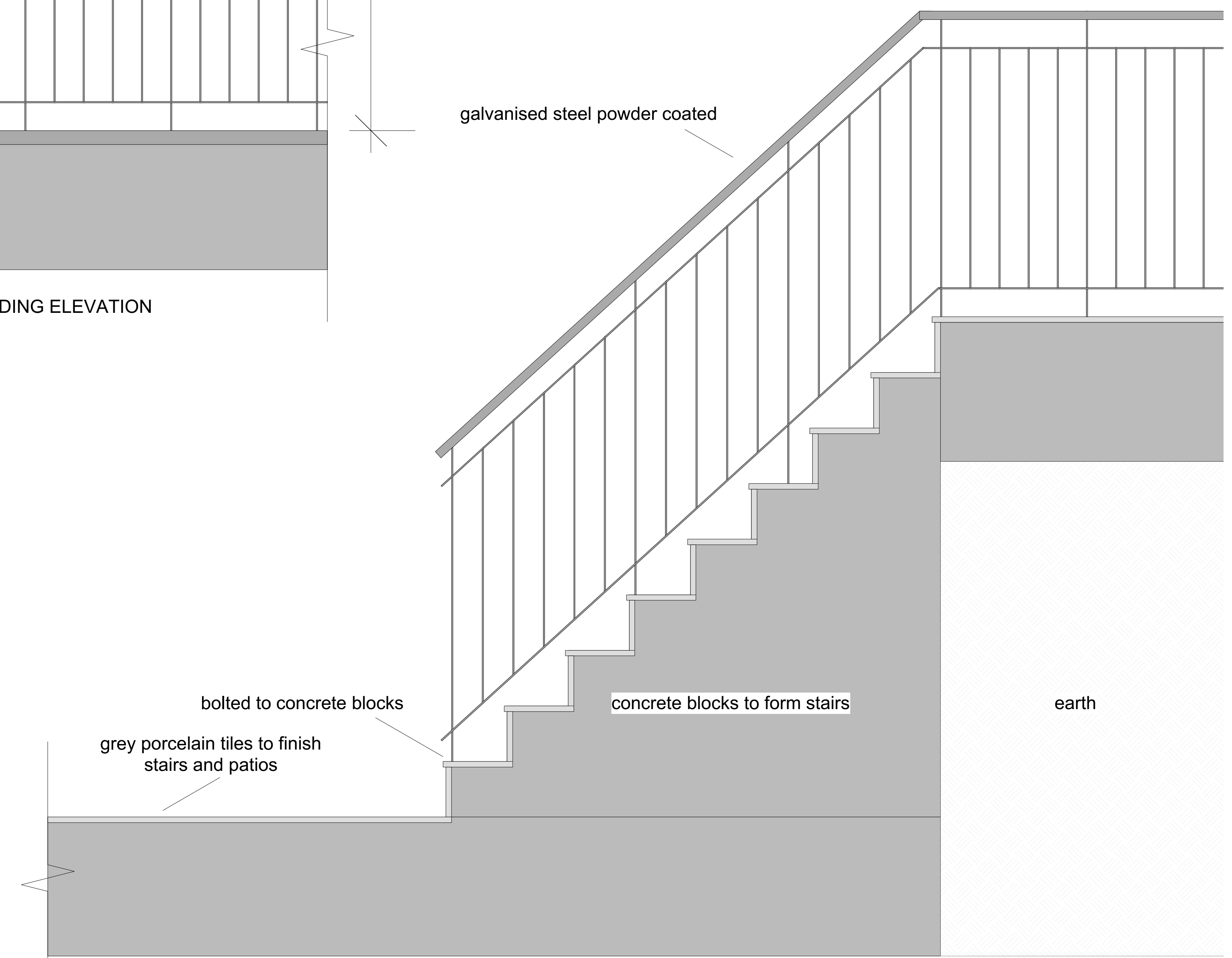
STAIRS WITH BALUSTRADING ELEVATION
