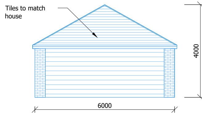
1 Front Elevation Scale 1:100
