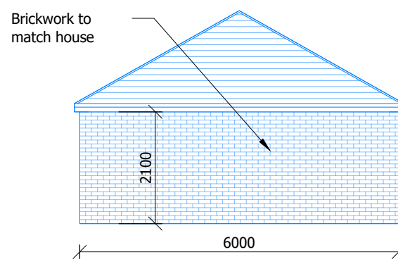
2 Side Elevations Scale 1:100
