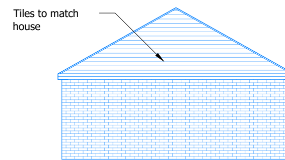
3 Rear Elevation Scale 1:100
