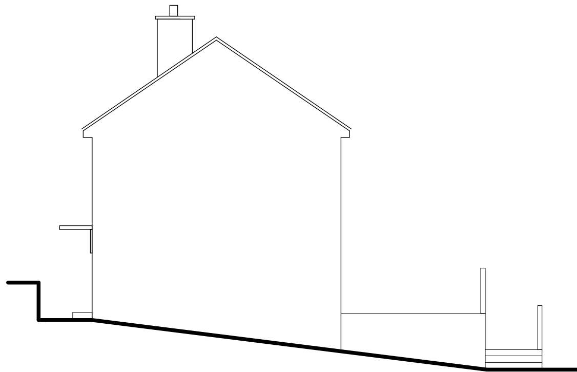
4 PROPOSED SIDE ELEVATION 03 SCALE 1:50 @A2
