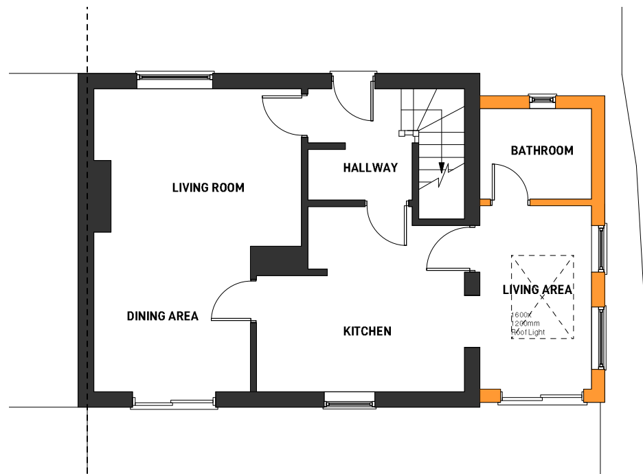
2 PROPOSED GROUND FLOOR 01 SCALE 1:100 @A3
