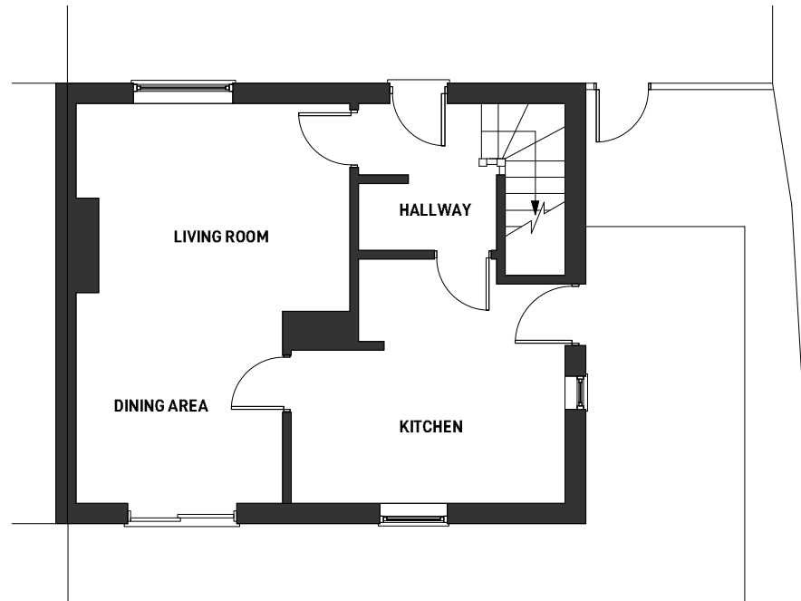
01 EXISTING GROUND FLOOR 01 SCALE 1:50 @A2
