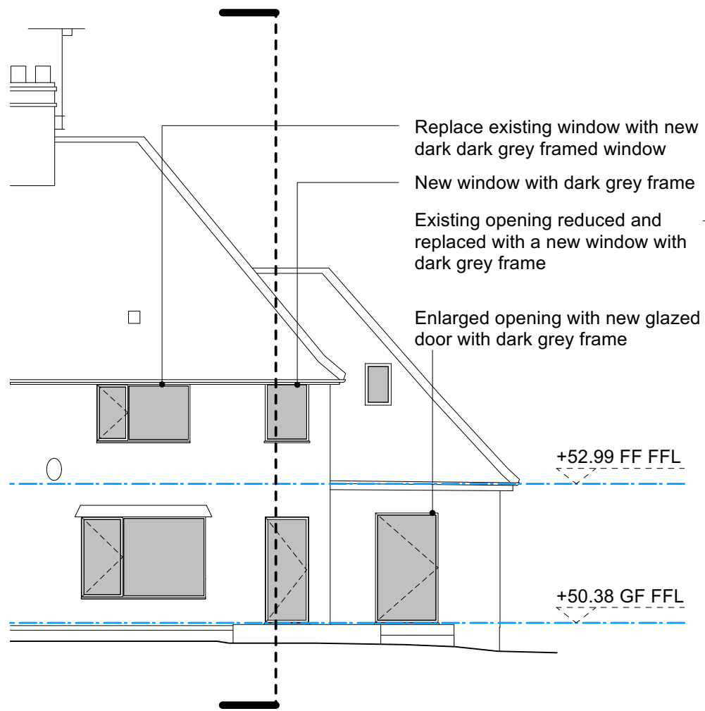
307.04 - PROPOSED SOUTH ELEVATION
