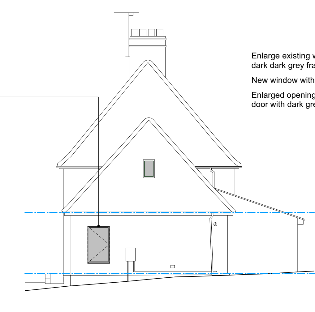
307.05 - PROPOSED EAST ELEVATION
