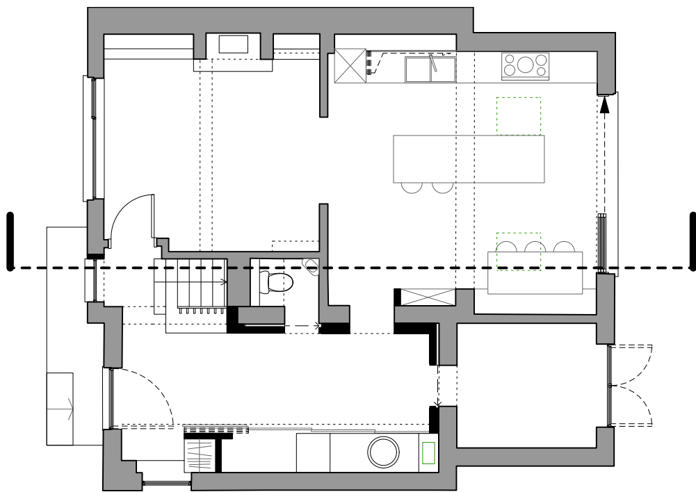
307.01 - PROPOSED GROUND FLOOR PLAN
