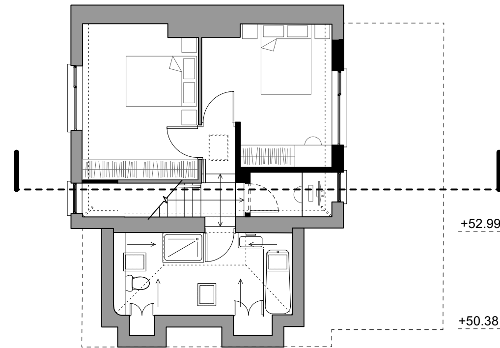
307.02 - PROPOSED FIRST FLOOR PLAN
