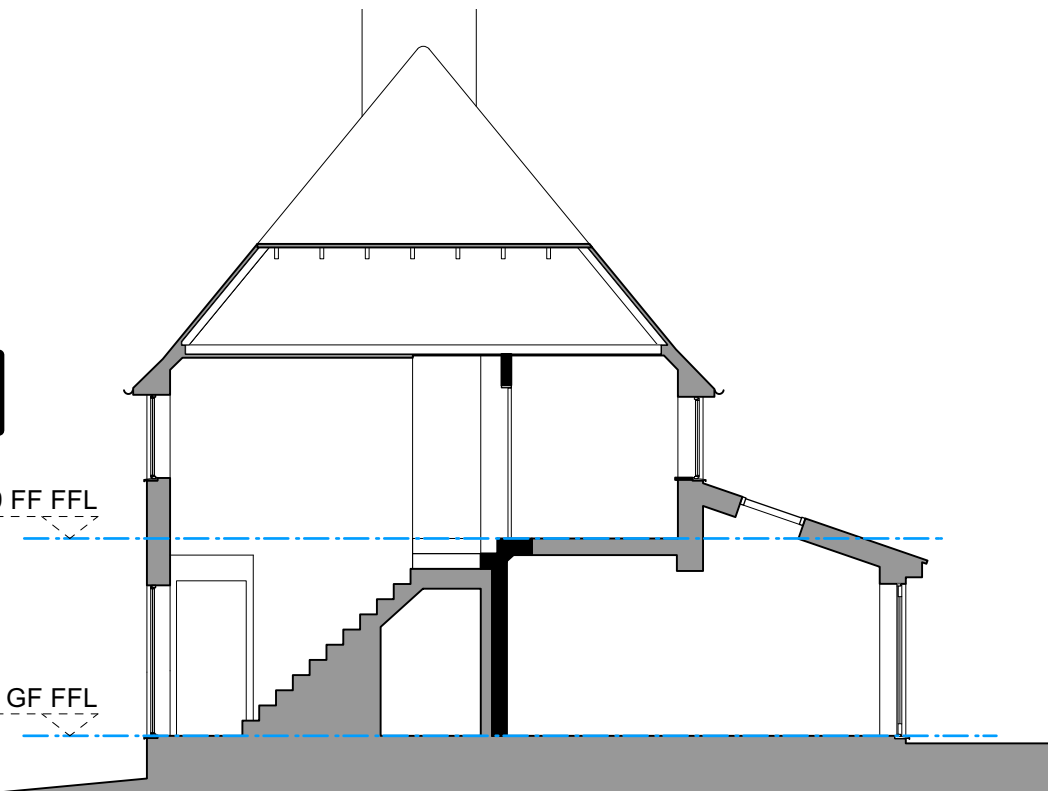
007.03 - PROPOSED SECTION
