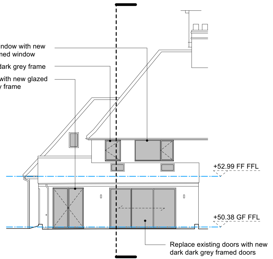
307.06 - PROPOSED NORTH ELEVATION
