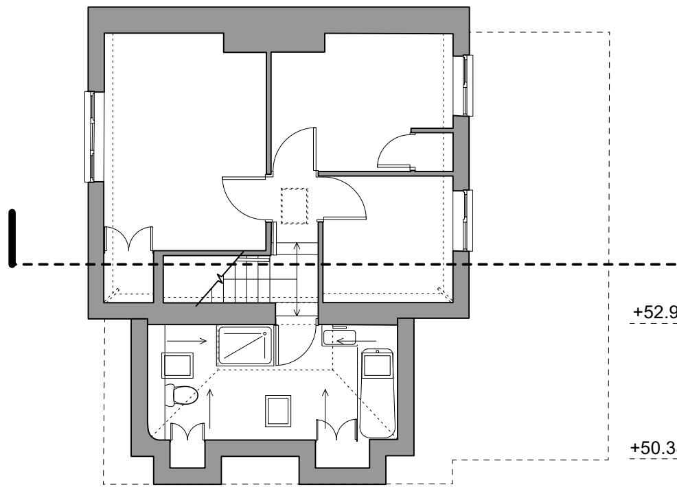
007.02 - EXISTING FIRST FLOOR PLAN
