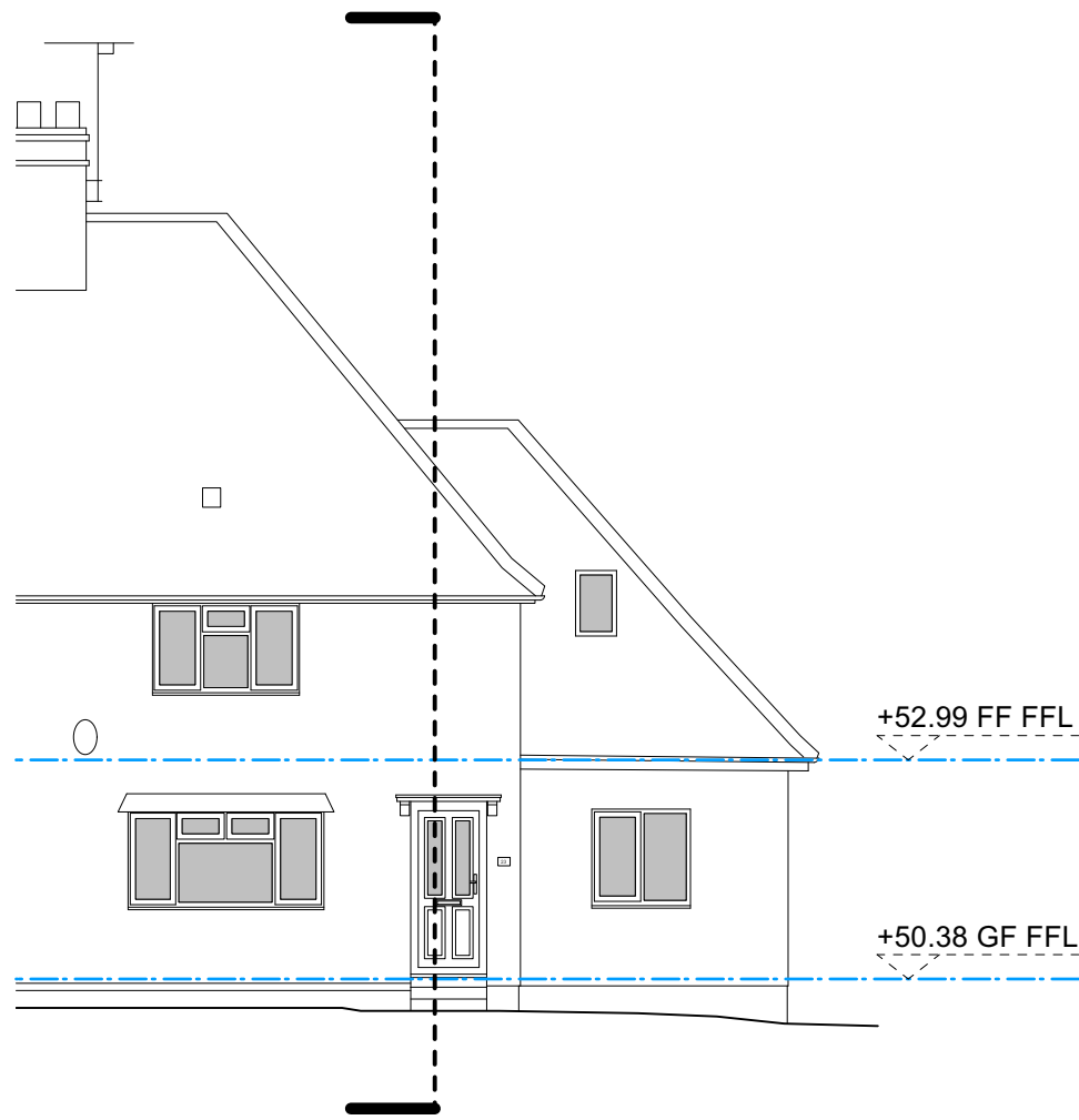
007.04 - EXISTING SOUTH ELEVATION
