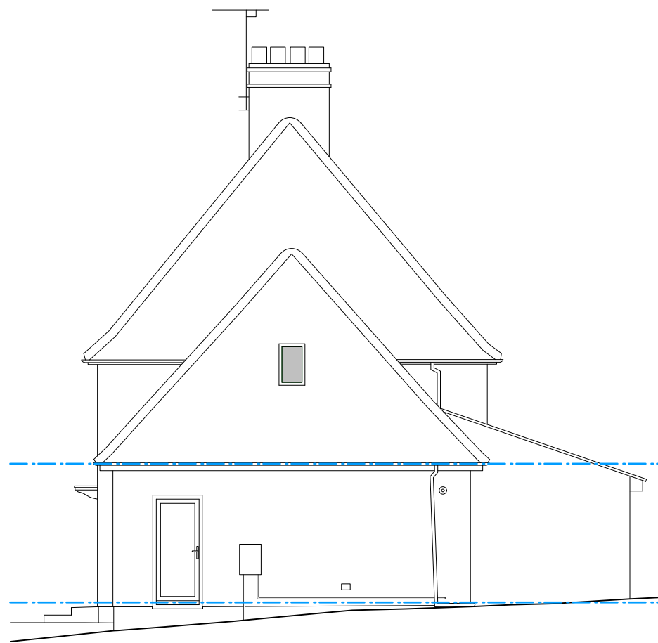
007.05 - EXISTING EAST ELEVATION
