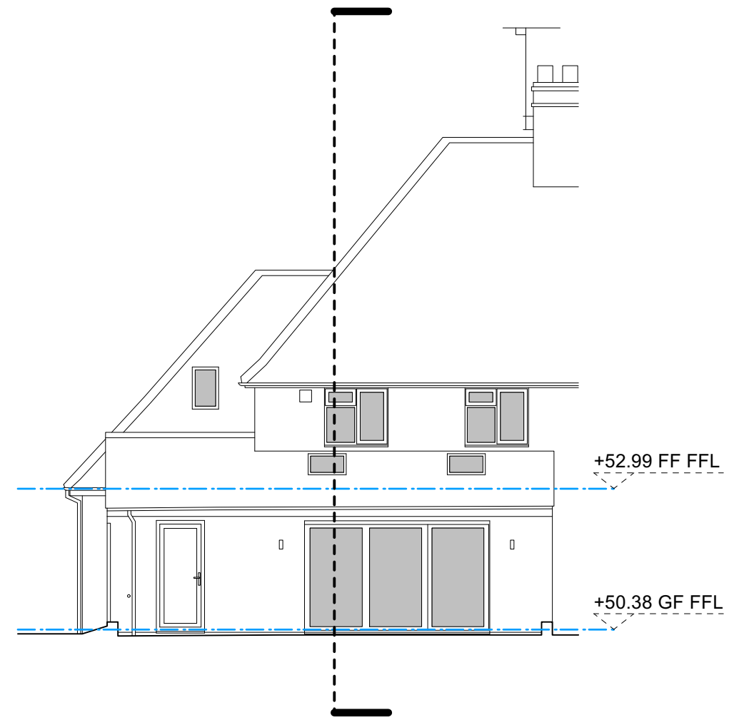
007.06 - EXISTING NORTH ELEVATION
