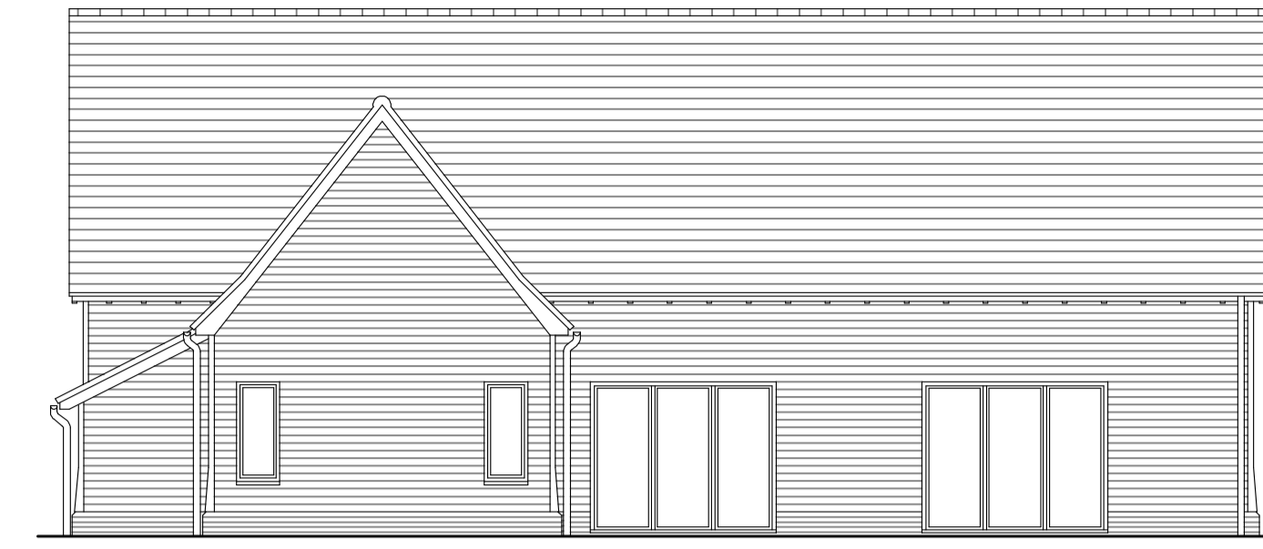
1:100 REAR ELEVATION (North-West) 0 1 2 3 4 5m Scale Bar
