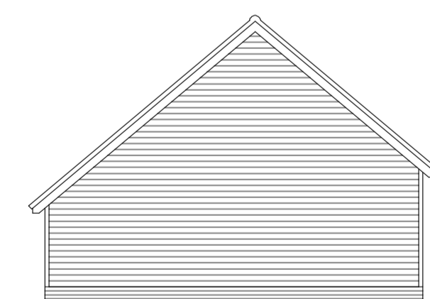
1:100 Side Elevation
