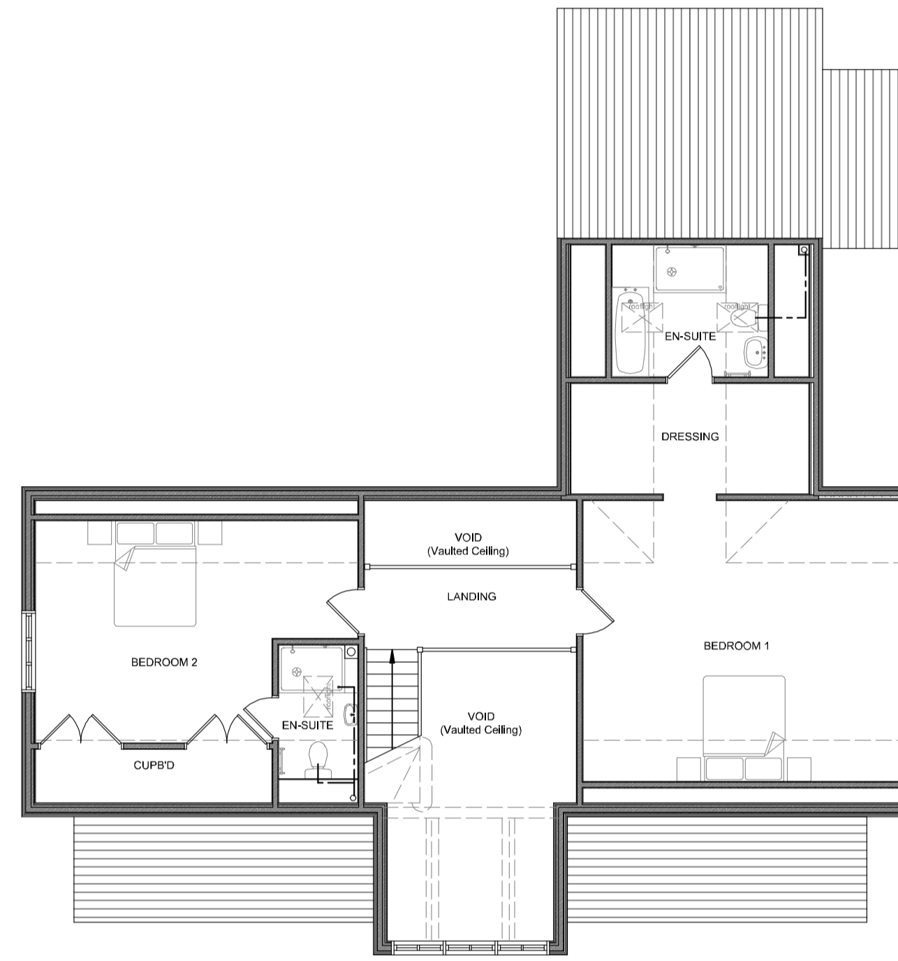
1:100 FIRST FLOOR PLAN 0 1 2 3 4 5m Scale Bar
