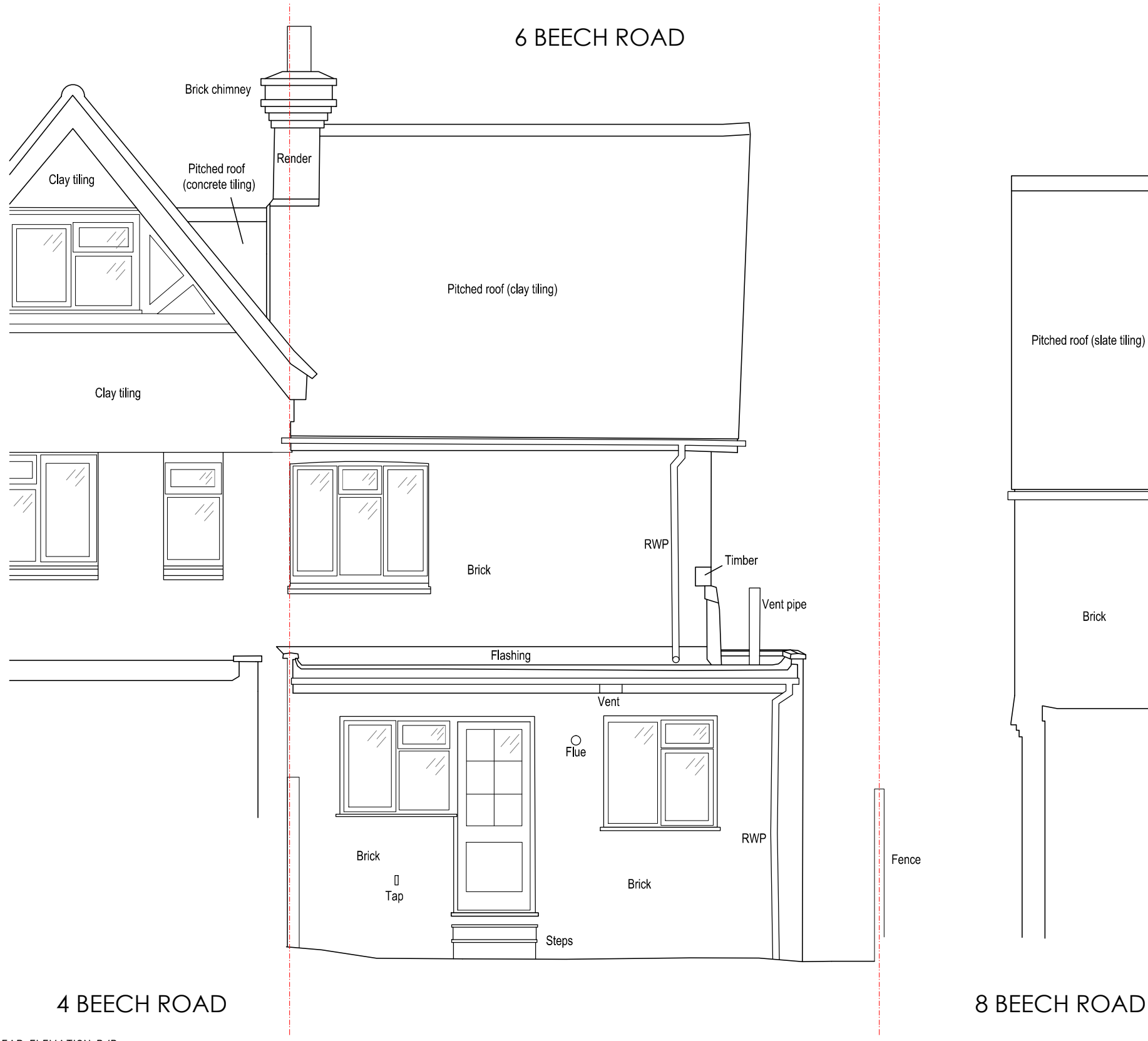
EXISTING REAR ELEVATION B/B SCALE 1:100
