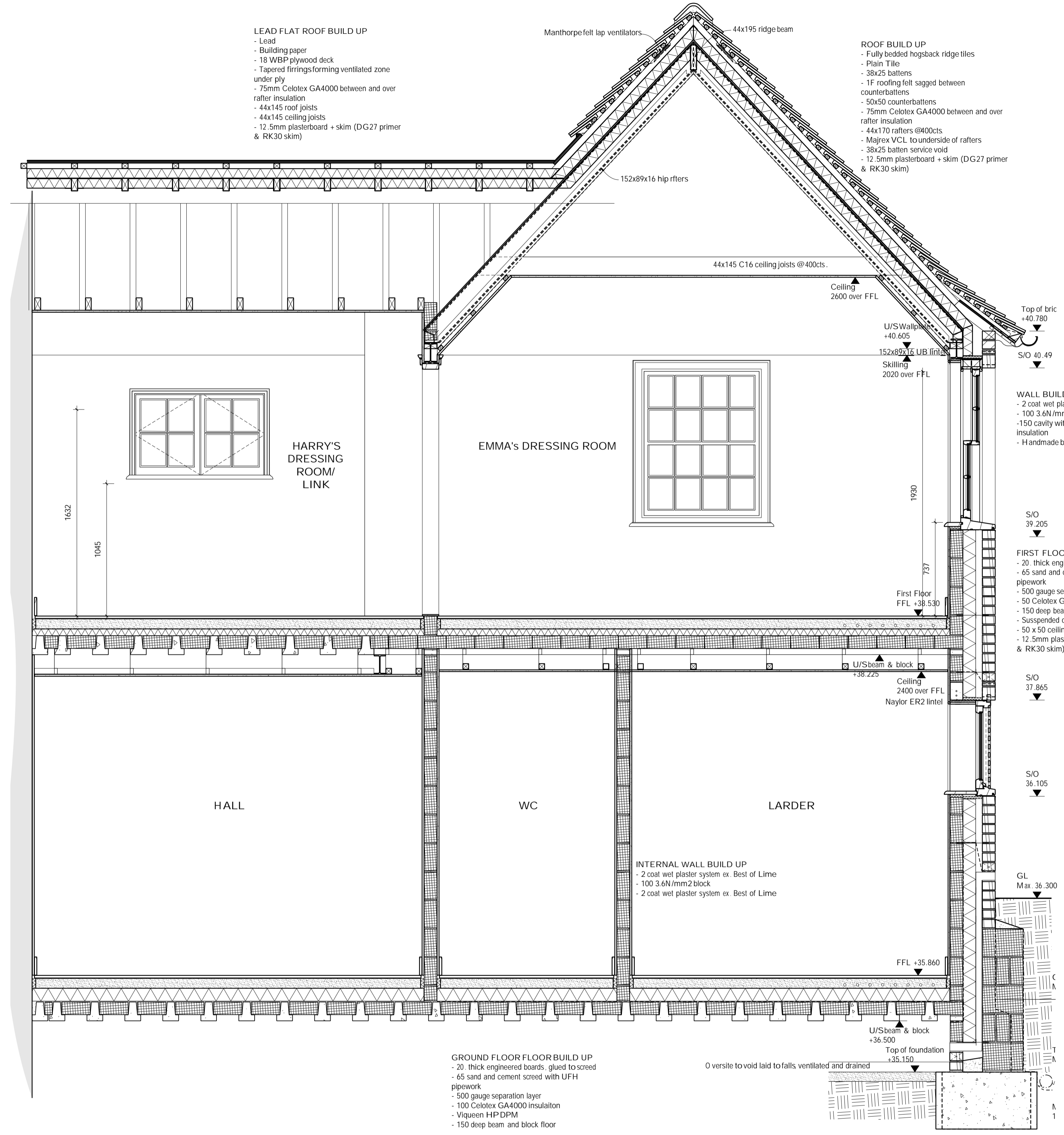
2 DETAIL SECTION THROUGH DRESSING ROOMS 1:20
