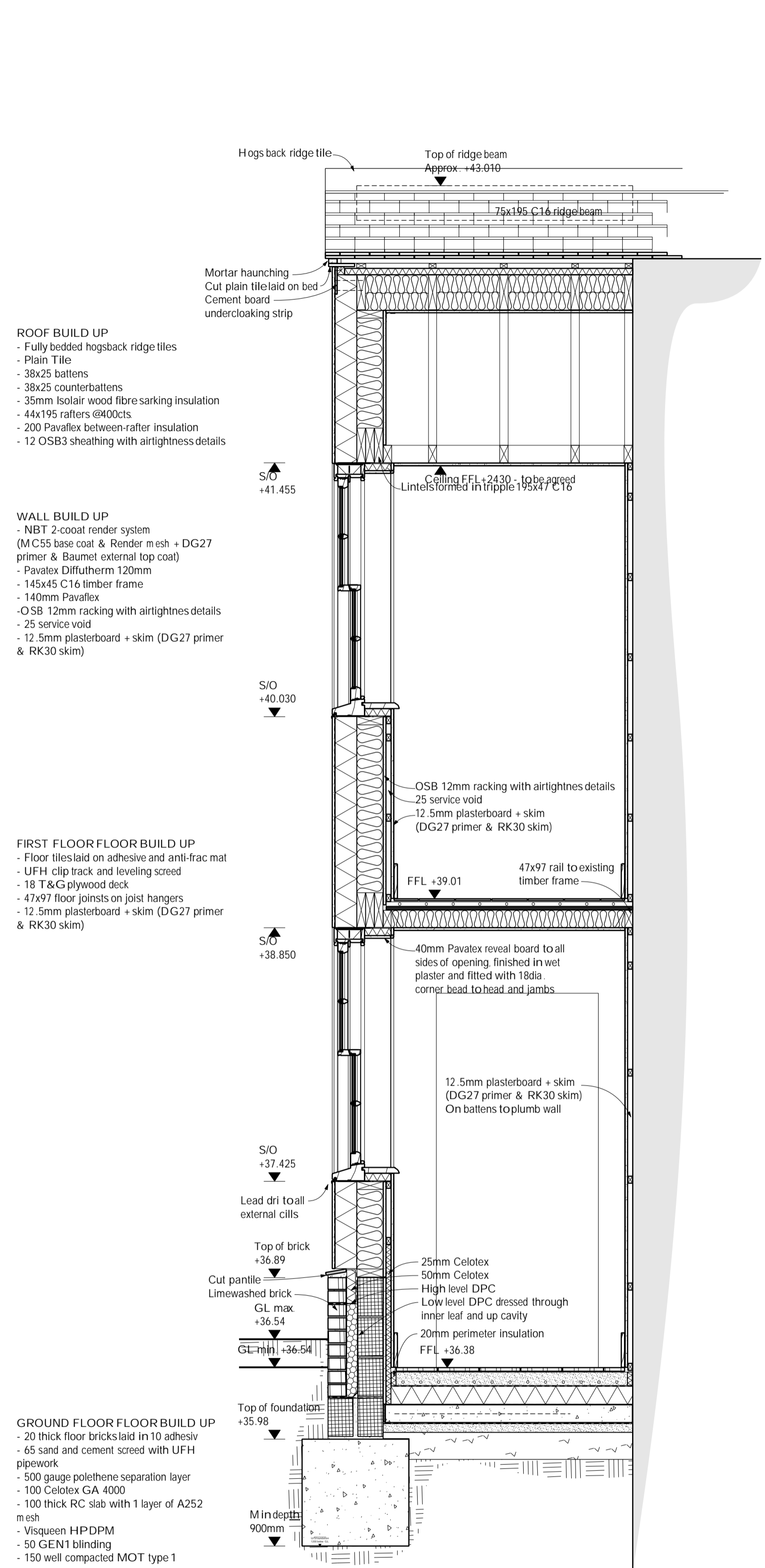
1 DETAIL SECTION THROUGH NW EXTENSION 1:20
