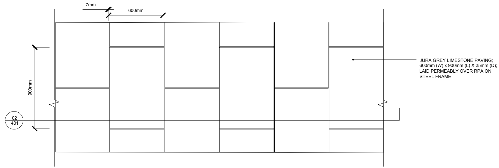
01 TYPICAL PAVING DETAIL WITHIN RPA 401 PLAN SCALE 1:20
