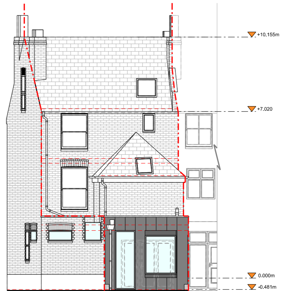
Rear Elevation
