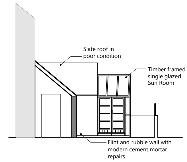
EXISTING SECTION A-A
