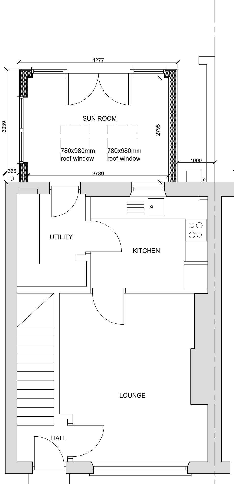
PROPOSED GROUND FLOOR PLAN. 1 : 50.
