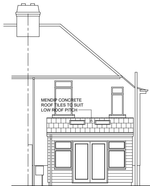
PROPOSED REAR (WEST) ELEVATION. 1 : 100.
