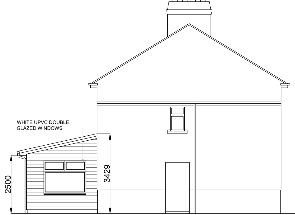
PROPOSED SIDE (SOUTH) ELEVATION. 1 : 100.
