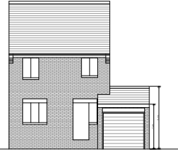
Rear Elevation As Proposed
