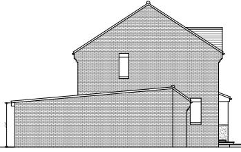
L Side Elevation As Proposed
