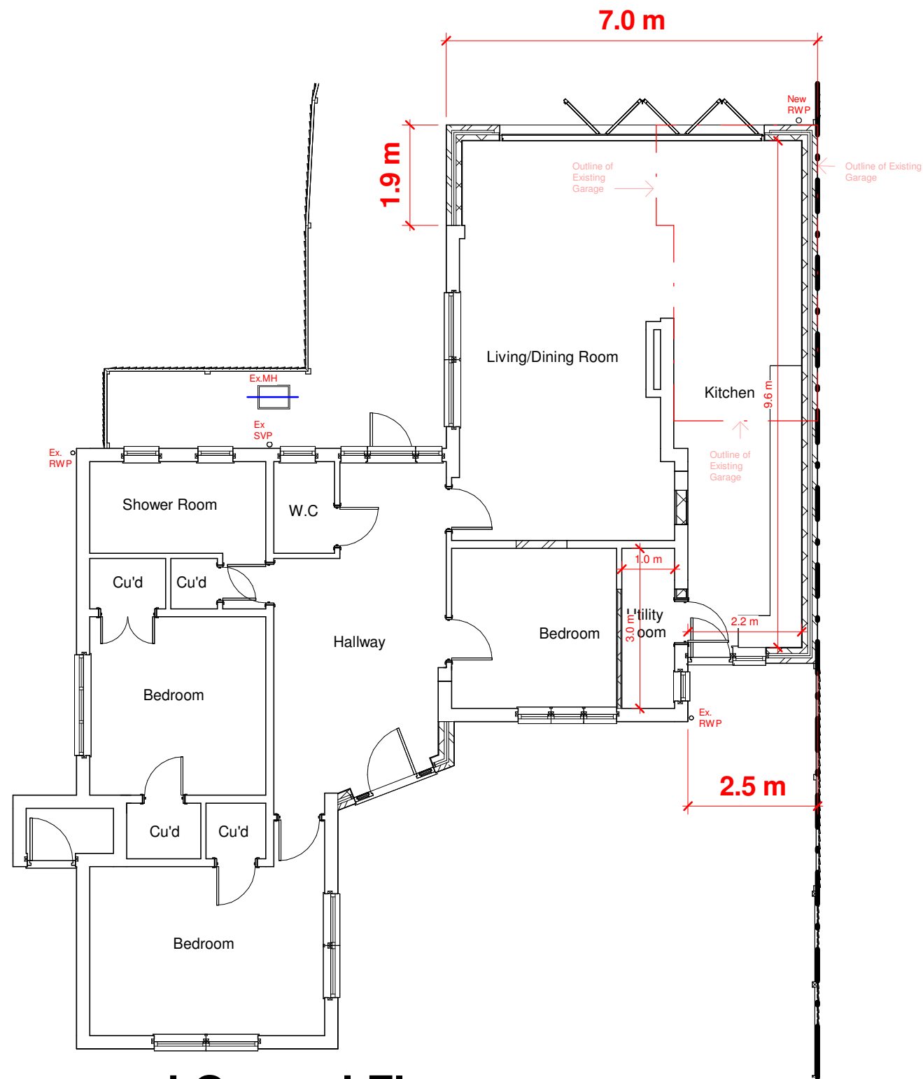
1 Proposed Ground Floor.
