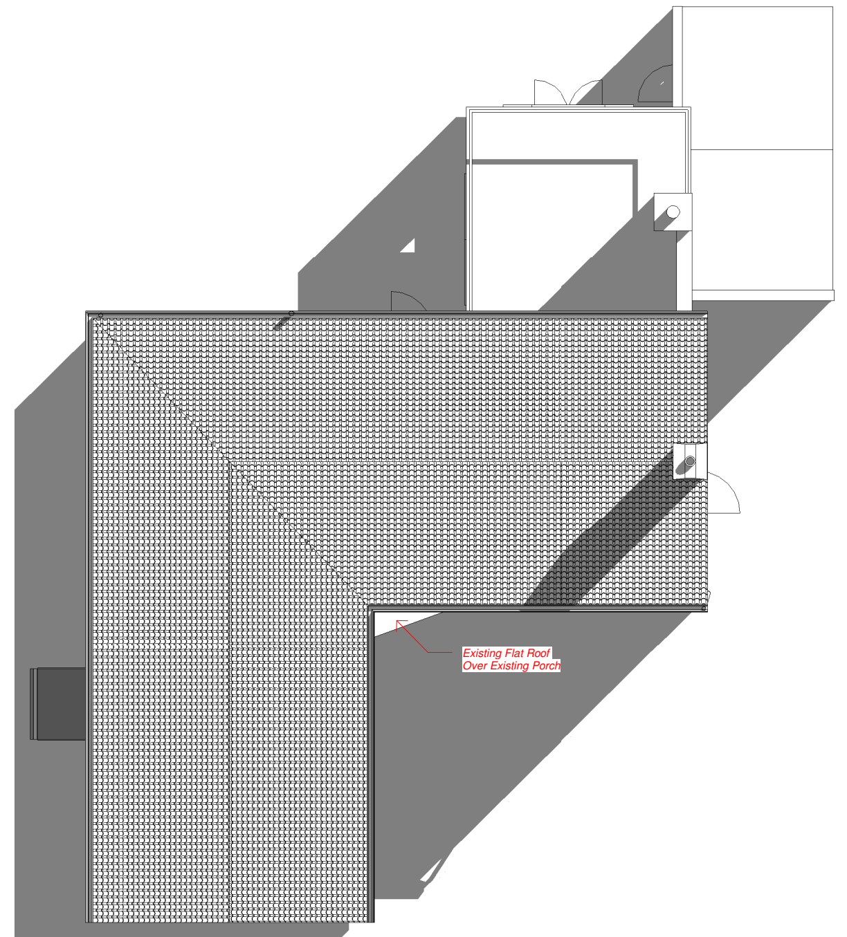
2 Existing Roof Plan. 1 : 100
