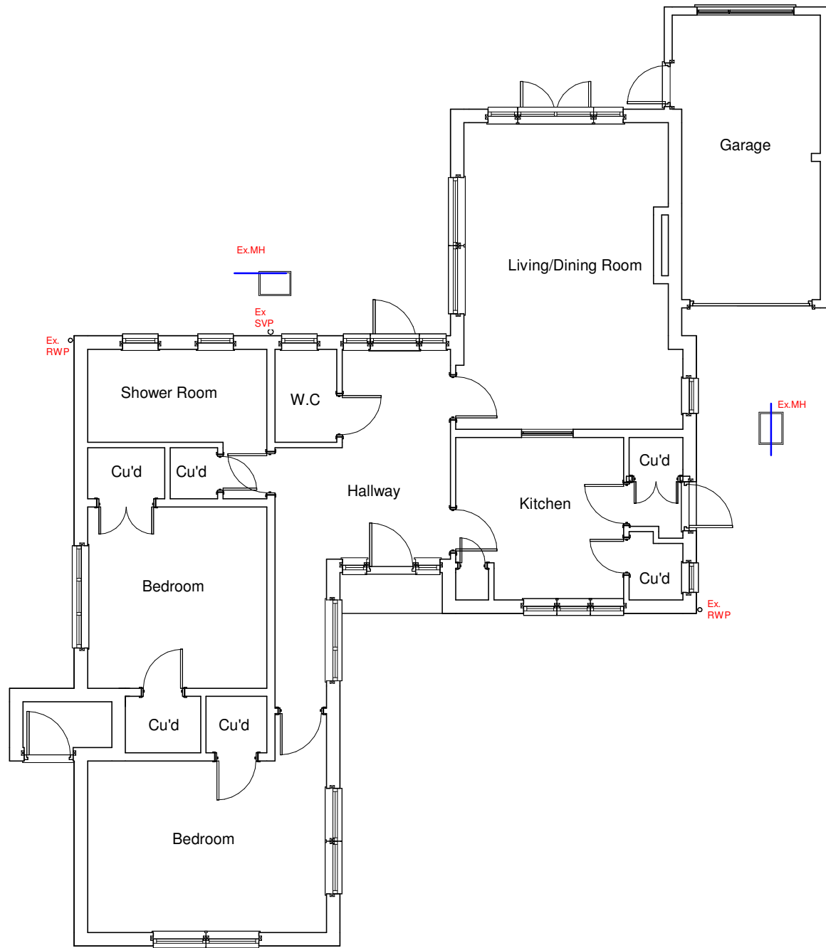
1 Existing Ground Floor. 1 : 100
