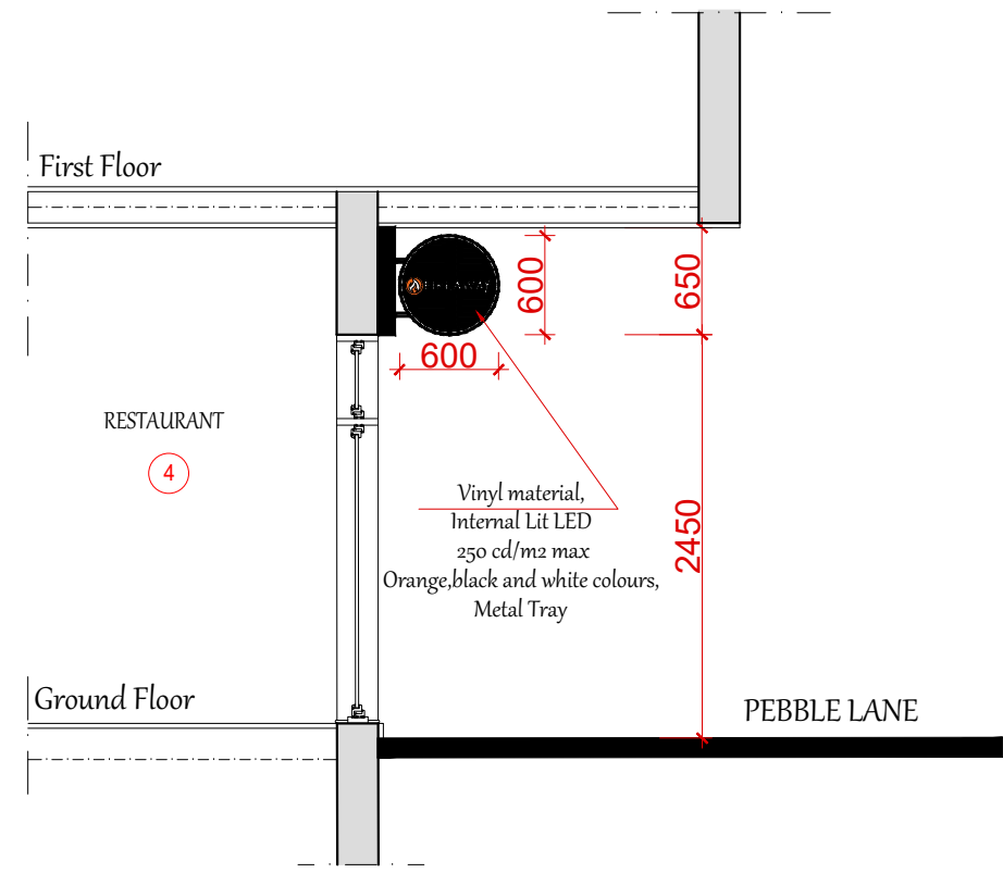
PROPOSED FRONT SECTION(SIGN DETAIL) SCALE: 1/50 @A3
