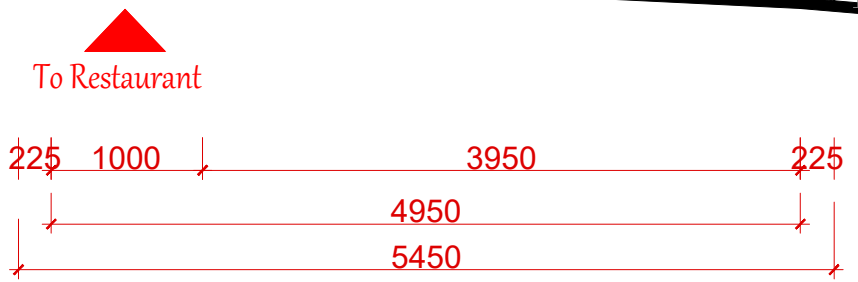
PROPOSED FRONT ELEVATION SCALE: 1/50 @A3
