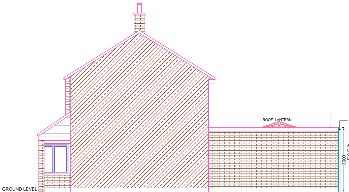
PROPOSED ELEVATION SIDE A
