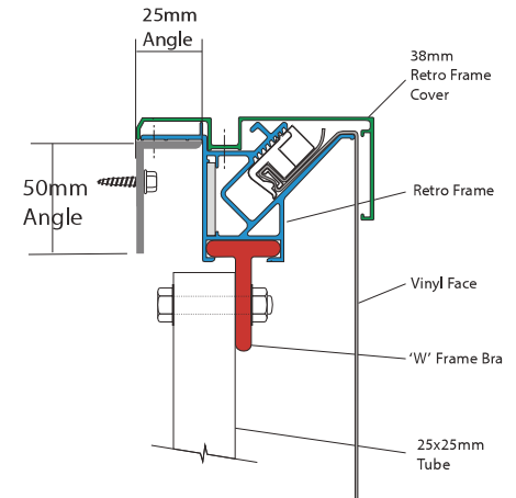
Generic Section for Retroframe Non-Illuminated
