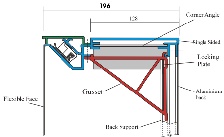
General Box Profile
