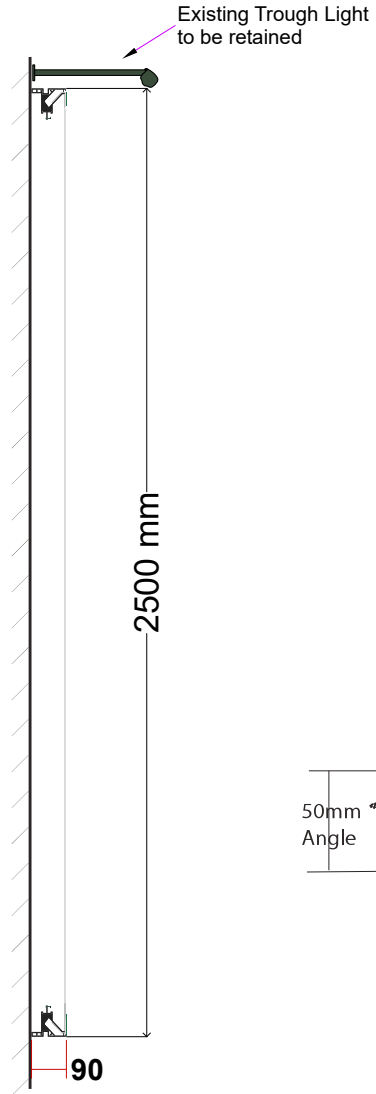
Section for Retroframes Signs 2a/2b
