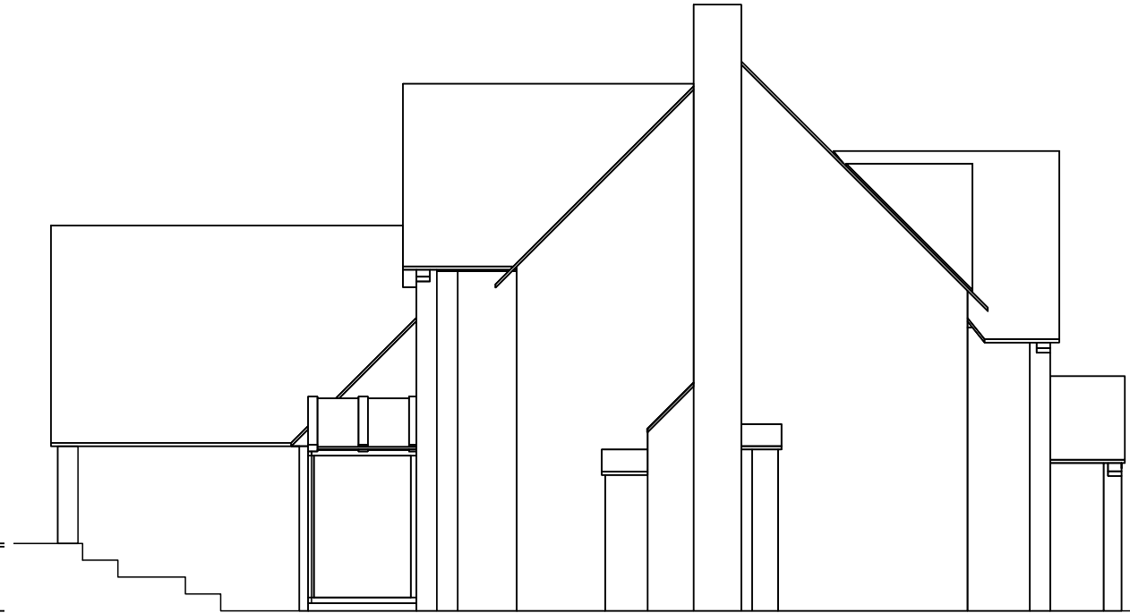
EXISTING WEST ELEVATION - 1:100
