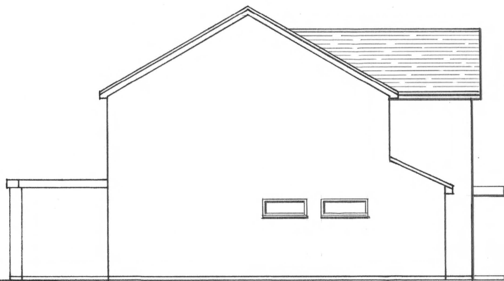
LEFT ELEVATION
