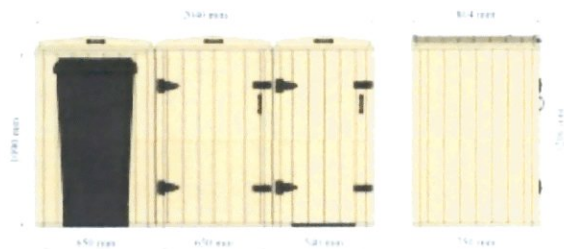
Helius Triple Wheelie Bin Storage for 2 x 180 Litre Bins and 1 x 140 Litre Wheelie Bin Dimensions
