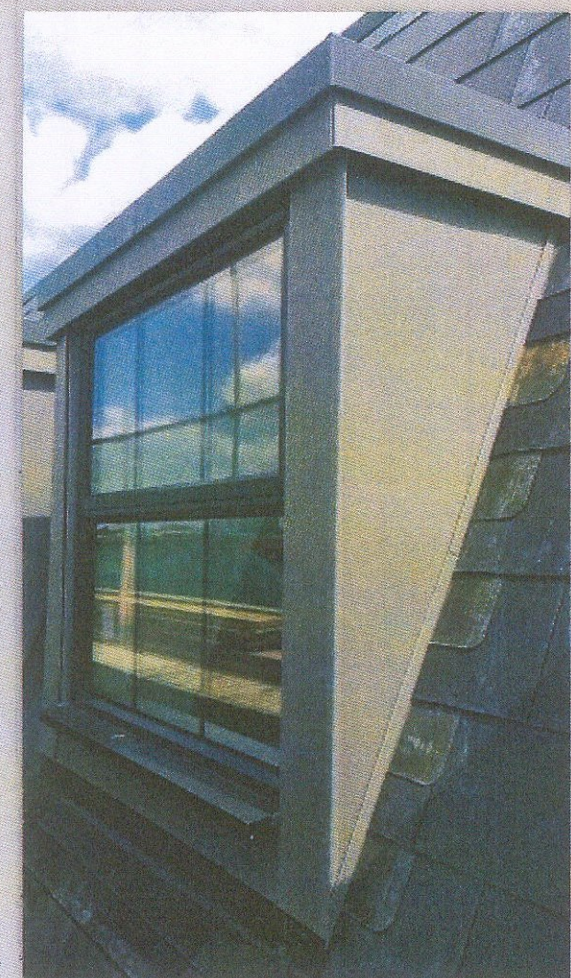
PROPOSED DORMER CHEEKS CLADDING
