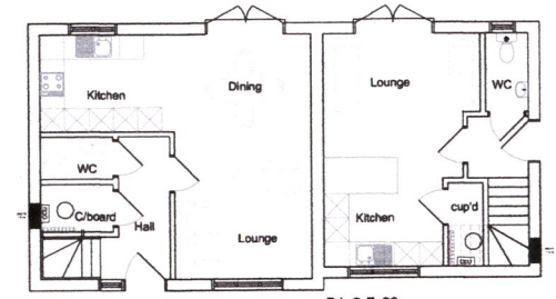
PLOT 25 GIA: 81sqm PLOT 26 GIA: 58sqm
