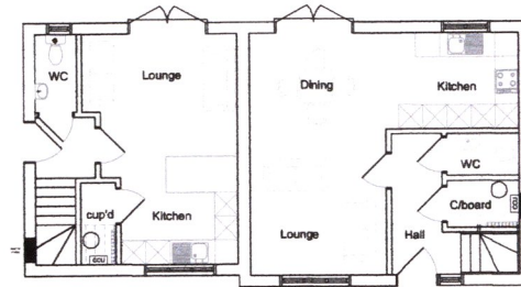
PLOT 23 GIA: 58sqm PLOT 24 GIA: 81sqm
