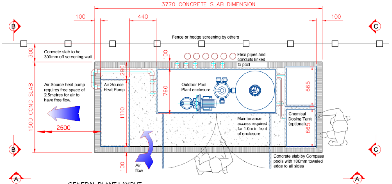
GENERAL PLANT LAYOUT
