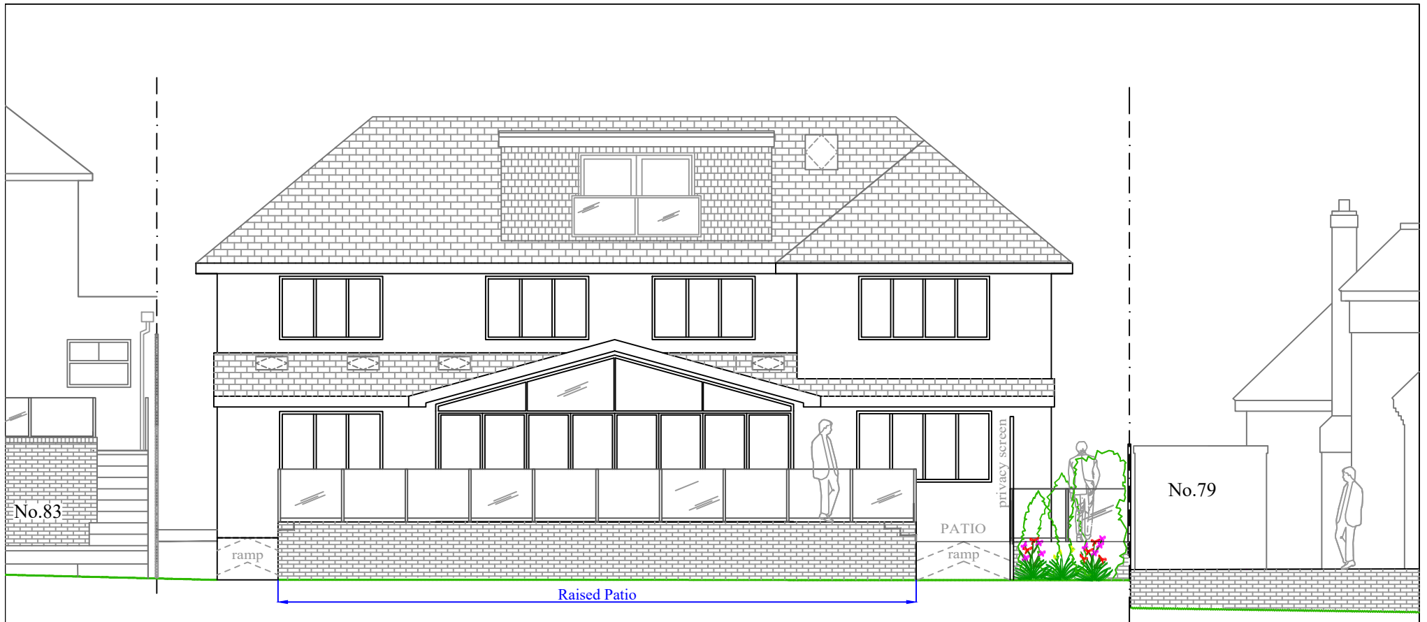
REAR ELEVATION Retained as existing
