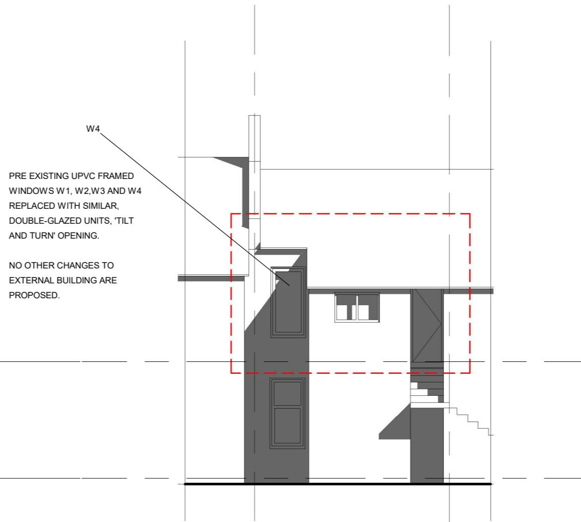
WEST (REAR) ELEVATION
