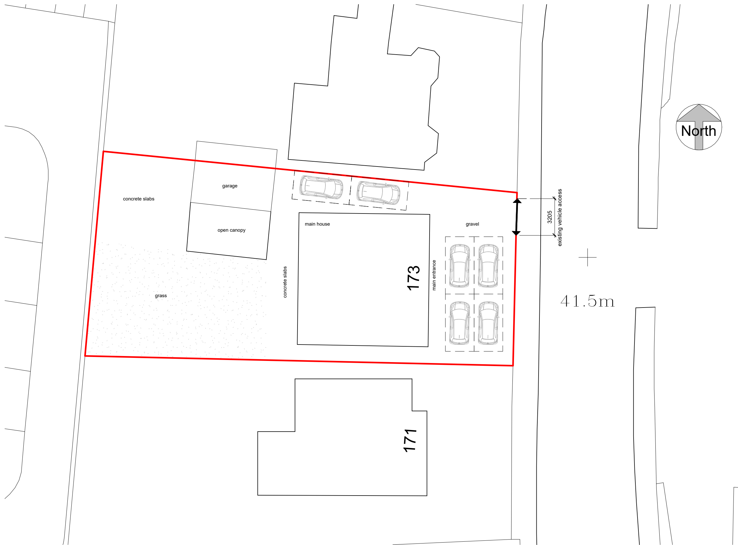
Site Plan as Existing 1 : 200
