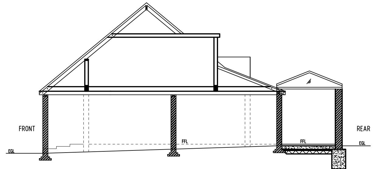
PROPOSED SECTION
