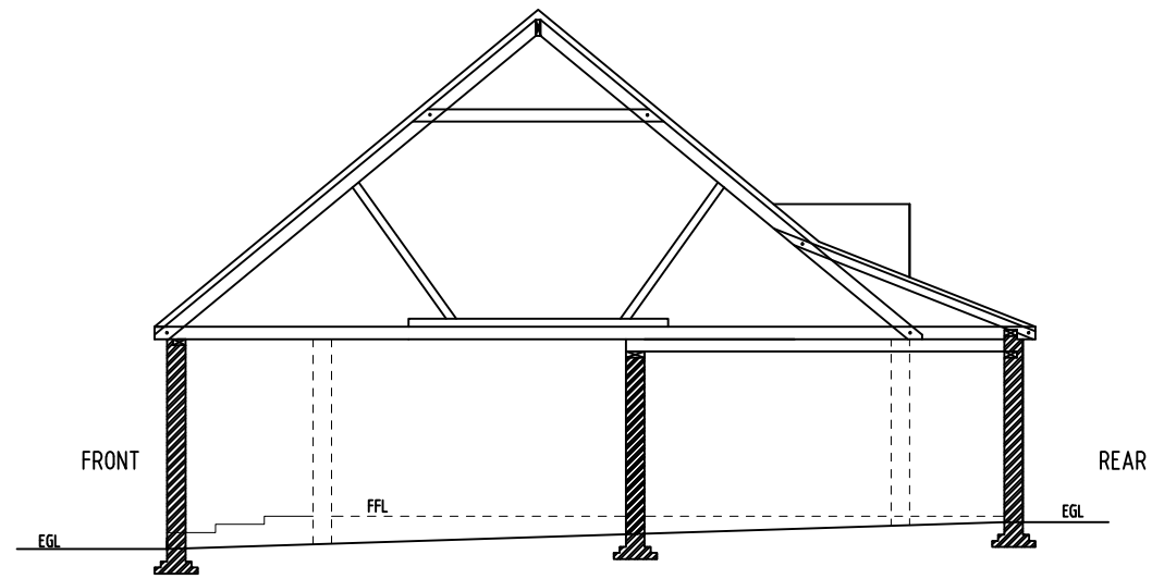
EXISTING SECTION
